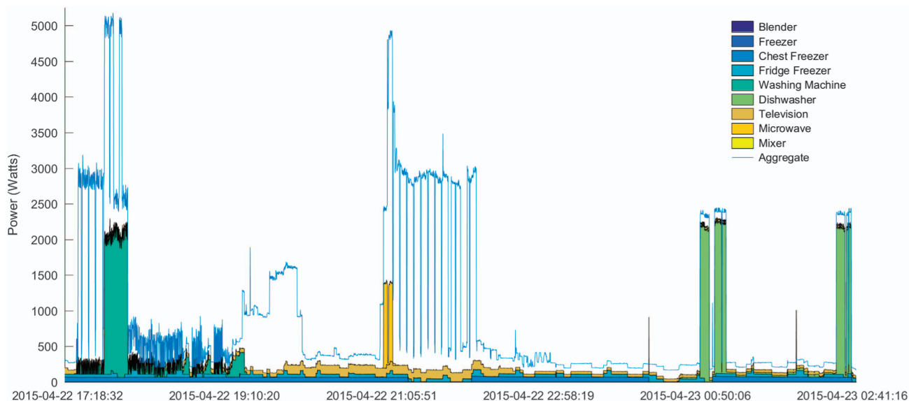
Figure 4. Power demand for House 10 during the evening of April 22nd 2015. The gap between the stacked IAM plot and the aggregate represents the power consumed by other appliances not monitored by IAMs.
