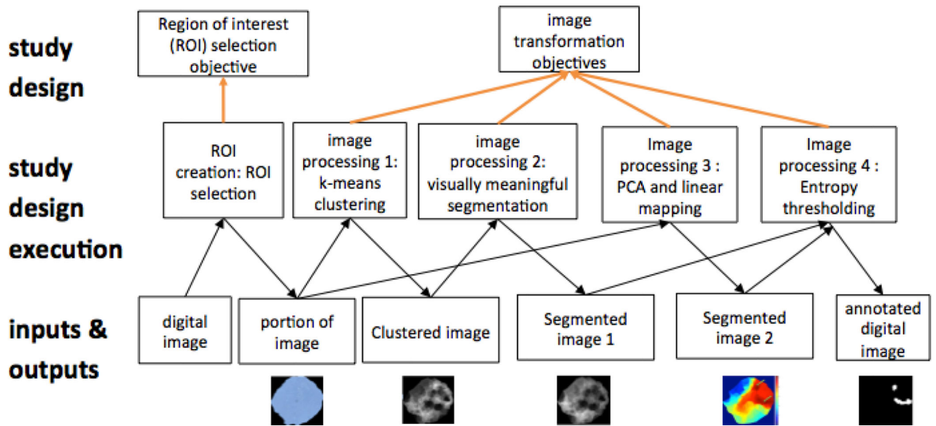
Figure 2. Sample workflow represented through QHIO and OBI terms. (PCA = Principal Component Analysis)
