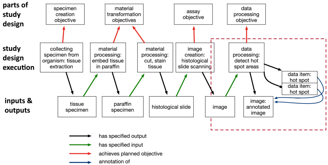
Figure 1. From specimen to hot spot detection. Overview of types and relationships in QHIO. Types are taken from OBI. More specific types from QHIO noted after colon.
