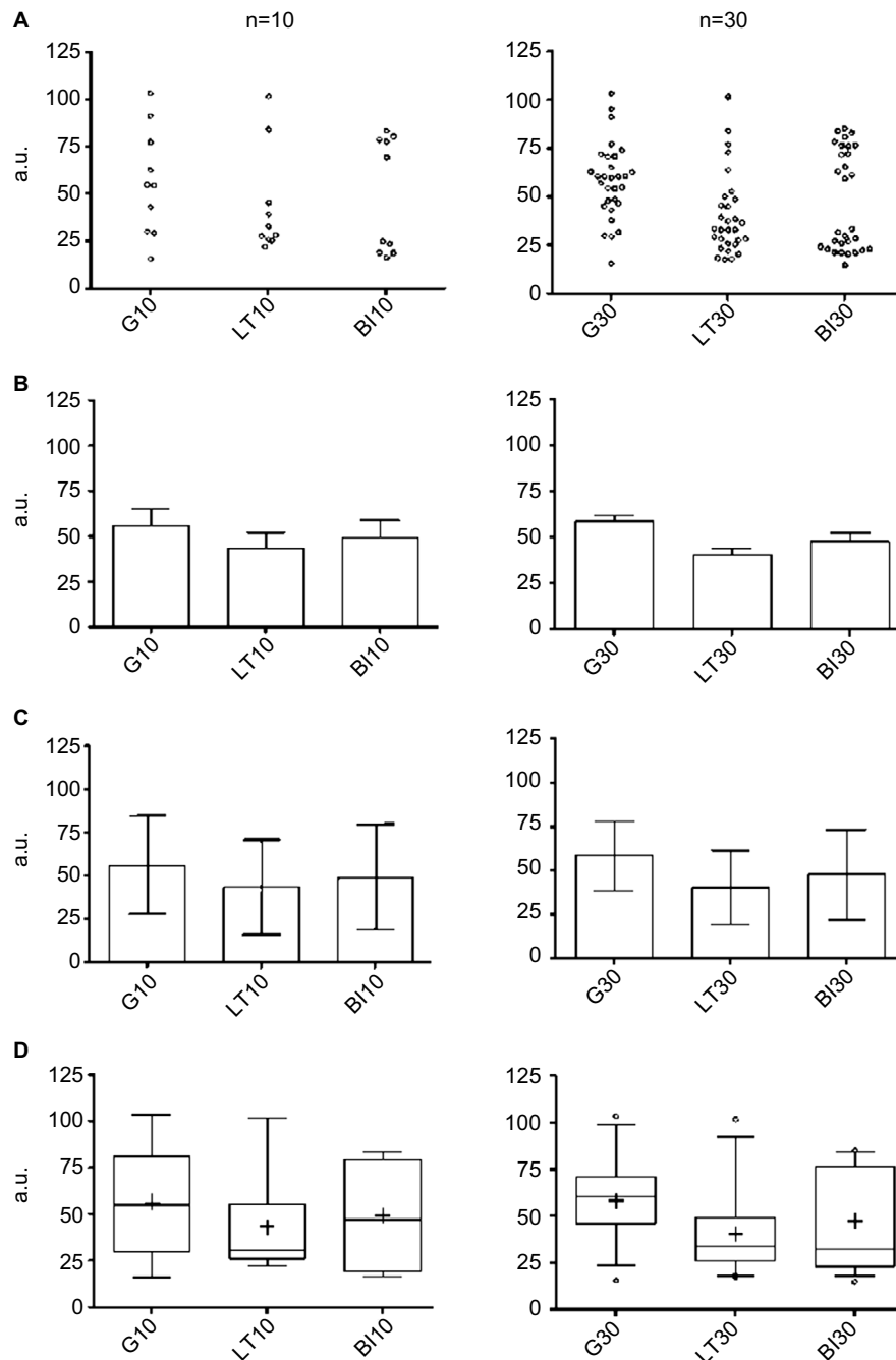
Figure 5 Plotting views of three common distributions.
