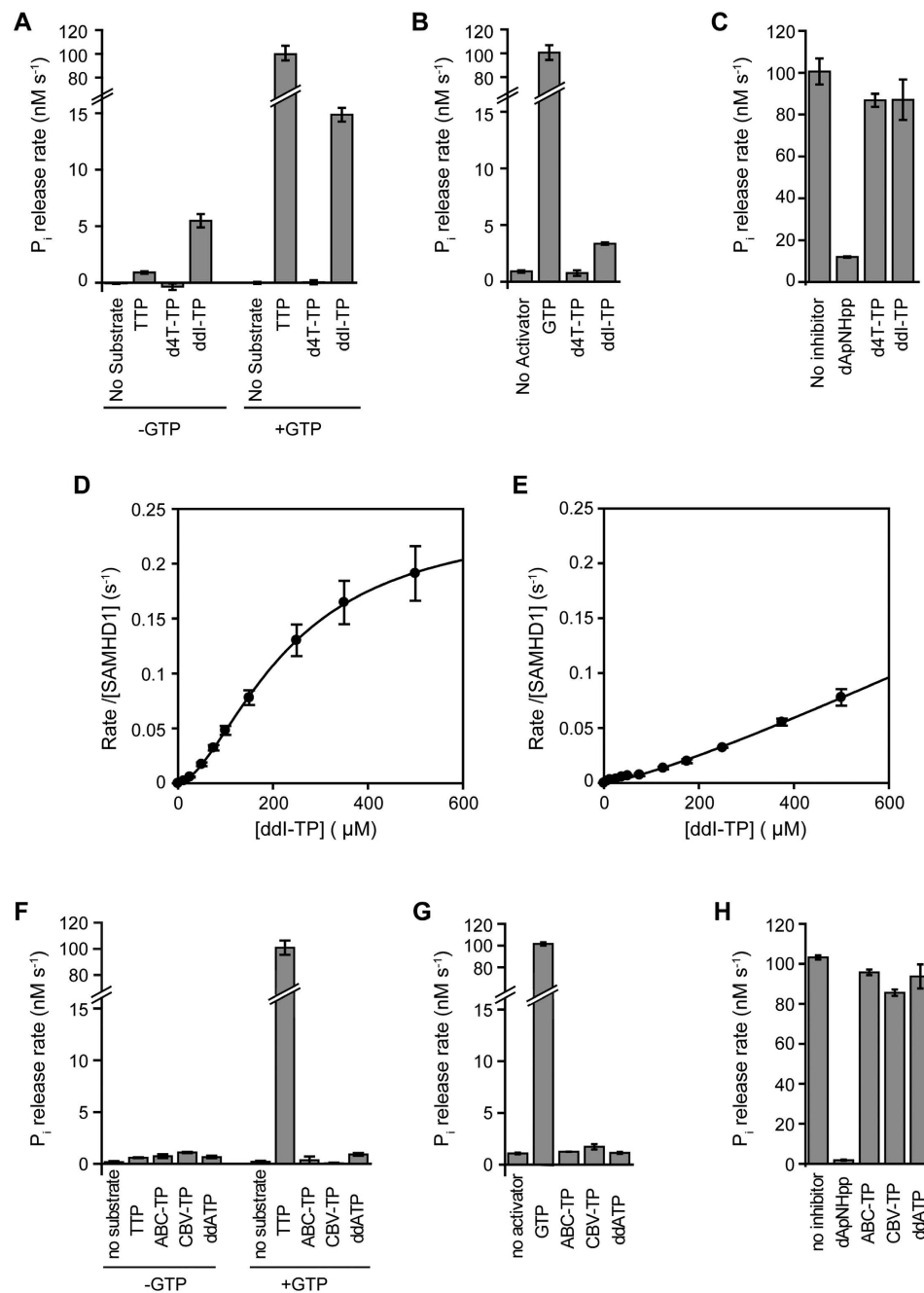
Figure 1. The effects of d4T-TP,ddl-TP,dda-TP, ABC-TP and CBV-TP on SAMHD1 triphosphohydrolyase activity. (A) Hydrolysis of 0.3 mM TTP, d4T-TP or ddl-TP in the absence (left) and presence (right) of 0.1 mM activator GTP. (B) Activation of SAMHD1 TTP hydrolysis. Triphosphohydrolyase activity was measured with 0.3 mM TTP substrate upon addition of 0.1 mM GTP, d4T-TP or ddl-TP as activators. (C) Inhibition of SAMHD1 GTP-activated TTP hydrolysis. Triphosphohydrolyase activity was measured with 0.3 mM TTP and 0.1 mM GTP activator alone and with addition of 0.3 mM dApNHpp positive control, d4T-TP or ddl-TP. Error bars are the standard error of the mean (SEM) of three independent measurements. (D) Concentration dependence of SAMHD1 ddl-TP hydrolysis in the presence of 0.2 mM GTP (saturating activator concentration). Nonlinear least squares fitting using a Hill equation gives the apparent binding constant K_S = 226 \pm 12 \mu\text{M} , catalytic constant k_{cat} = 0.24 \pm 0.04 \text{ s}^{-1} and the Hill coefficient n = 1.7 \pm 0.1 (Mean \pm SEM). (E) ddl-TP allosteric activation of TTP hydrolysis. Rates were determined for 1 mM TTP at varying dd-I-TP concentration. Nonlinear least squares fitting gives only lower estimates for the maximal rate and the ddl-TP concentration at half maximal activation of k_{max} > 0.1 \text{ s}^{-1} and K_a > 300 \mu\text{M} . (F) Hydrolysis of 0.3 mM TTP, ABC-TP, CBV-TP and ddATP in the absence (left) and presence (right) of 0.1 mM activator GTP. (G) Activation of SAMHD1 TTP hydrolysis. Triphosphohydrolyase activity was measured with 0.3 mM TTP substrate upon addition of 0.1 mM GTP, ABC-TP, CBV-TP or ddATP as activators. (H) Inhibition of SAMHD1 GTP-activated TTP hydrolysis. Triphosphohydrolyase activity was measured with 0.3 mM TTP and 0.1 mM GTP activator alone and with addition of 0.3 mM dApNHpp positive control, ABC-TP, CBV-TP or ddATP. Error bars are the range of data from two independent measurements.
