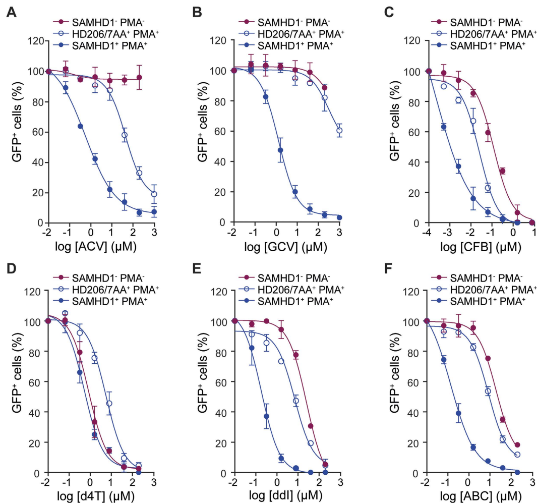
Figure 3. Anti-HIV-1 activities of nucleoside analogues in U937 cells expressing SAMHD1. Antiviral activities were determined in undifferentiated (PMA - ) and differentiated (PMA + ) U937 cells expressing SAMHD1 or the mutant HD206-7AA. Cells were cultured in the presence of increasing concentration of Aciclovir (ACV) (A), Ganciclovir (GCV) (B), Clofarabine (CFB) (C), Stavudine (d4T) (D), Didanosine (ddI) (E) and Abacavir (ABC) (F). Cells were incubated with HIV-1-GFP and the percentage of infected GFP + cells was measured by flow cytometry. PMA - cells expressing SAMHD1 (red filled circles), PMA + cells expressing the mutant HD206-7AA (blue open circles) and PMA + cells expressing SAMHD1 (blue filled circles) are shown. Infectivity data is plotted as the normalised percentage of GFP + cells against drug concentrations. Error bars represent the standard deviation from at least 2 independent experiments.
