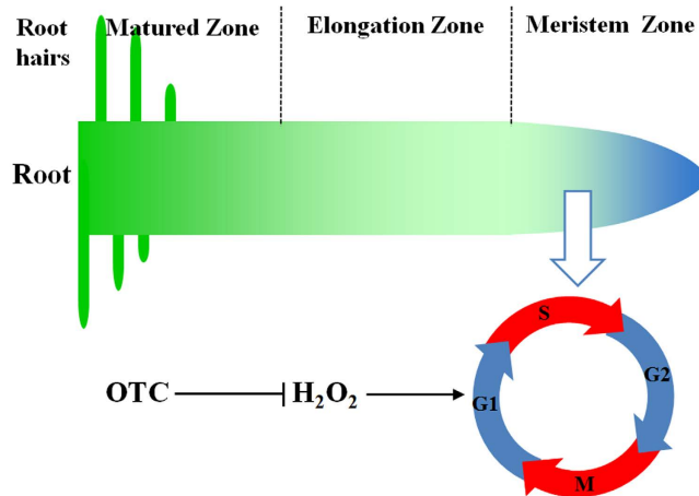
Figure 9. Model of the mechanism of inhibition of root growth by oxytetracycline (OTC) in tomato seedlings. OTC treatment results in a decline in H_2O_2 levels in root tips. H_2O_2 is a critical signal for maintaining the cell cycle in root meristem. Low H_2O_2 levels in the root tips as a result of OTC treatment lead to decreased root meristem size and root growth.
