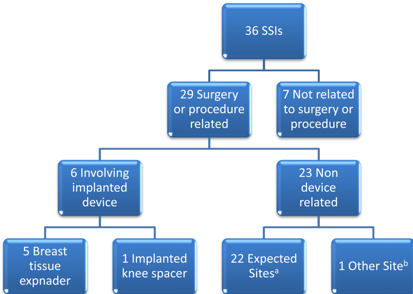
Figure 2. Details of S. lugdunensis skin and skin structure infection in cancer patients SSIs – skin and skin structure infections a - Expected sites included: breast – 15; inguinal, abdominal wall, perineal – 8; and axillary – 1 b - Other sites associated with mandibular surgery
