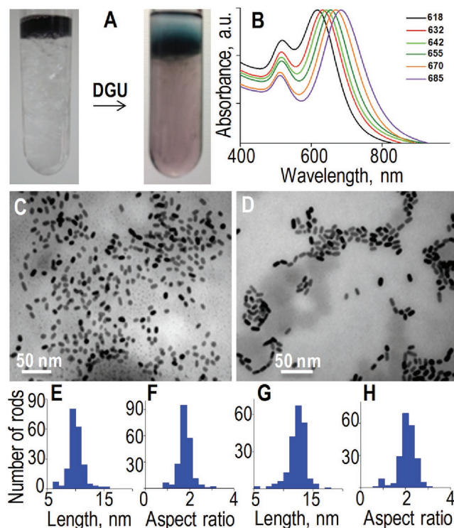
Figure 2. A) Photographs of DGU tube before and after centrifugation. B) UV/Vis absorption spectra of six fractions collected after DGU. C,D) TEM images of two fractions (618 and 642 nm peak absorption). E–H) The corresponding length and aspect ratio histograms are presented. They show average lengths of (E) 10 \pm 1 nm and (G) 13 \pm 1 nm with average aspect ratios of (F) 1.8 and (H) 2.2, respectively. Here, \approx 200 nanorods are used to construct histogram.
