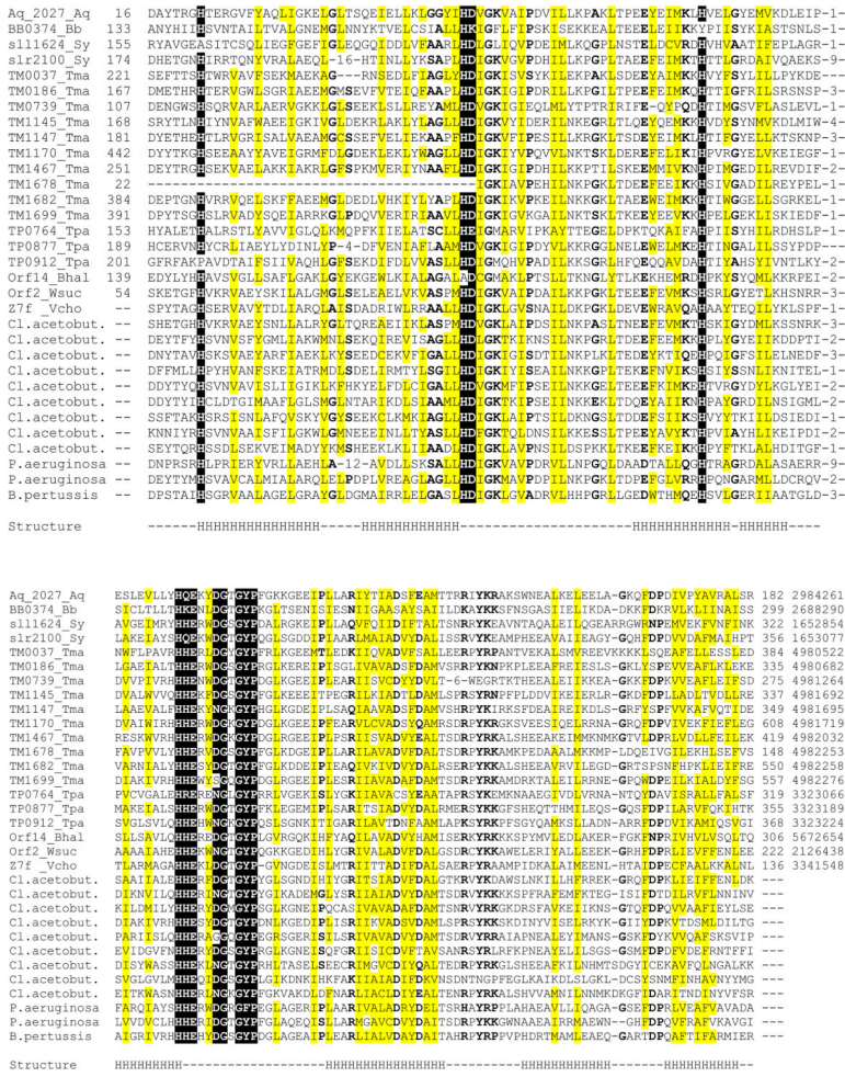
Figure 1. Multiple alignment of HD-GYP domains The proteins are listed under their names in complete genomes (left column) and their unique gene identification (gi) numbers in the GenBank protein database (right column); the numbers indicate positions of the first and the last residues in each protein, where available, and the distances between the aligned segments. Species name abbreviations are as follows: Aq, Aquifex aeolicus ; Bb, Borrelia burgdorferi ; Bhal, Bacillus halodurans ; Cl. acetobut., Clostridium acetobutylicum ; Sy, Synechocystis sp.; Tma, Thermotoga maritima ; Tpa, Treponema pallidum ; Vcho, Vibrio cholerae ; Wsuc, Wolinella succinogenes . Reverse shading indicates most conserved amino acid residues that are probably involved in metal and/or substrate binding. Grey shading indicates conserved uncharged amino acid residues, other conserved residues are in bold. The secondary structure of the HD domain is as predicted by PHDsec program (Rost and Sander, 1993); H indicates predicted \alpha -helical segments, dash indicates a loop or the absence of confident prediction.
