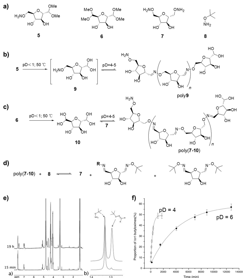
Figure 6. (a) Structures of ditopic monomers 5–7 and the termination agent 8. (b) Generation of the glycodamer poly9. (c) Generation of the glycodamer poly(7–10). (d) Dynamic chain termination: equilibrium upon addition of 8 to poly(7–10). (e) 1 H NMR spectra of the exchange mixture obtained after addition of 8 to poly(7–10) after 15 min and 19 h. (f) pD dependence of the rate of exchange between poly(7–10) and 8. Adapted with permission from ref 45. Copyright 2008 Wiley Periodicals, Inc.
