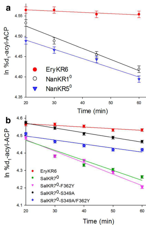
Figure 3. Time-dependent tandem EIX washout of deuterium from [2- 2 H]-6 by wild-type or mutant KR 0 domains.
