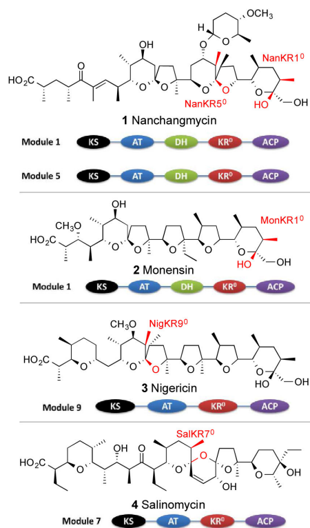
Figure 1. Representative polyethers and domain organization of the PKS modules that generate epimerized \alpha -methyl ketones, highlighted in red.
