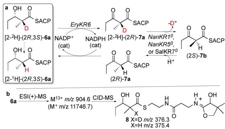
Scheme 4. Tandem EIX assay.
