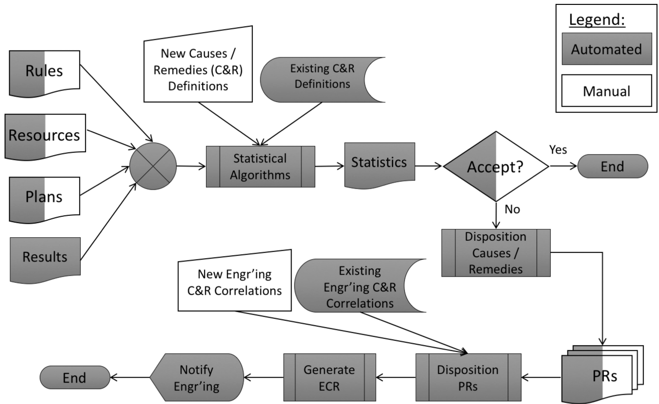
Fig. 5. Example process for Automated Engineering Change Requests to show how data is first aggregated together, statistical anomalies detected, engineering-design problems discovered, and engineering changes requests generated.
