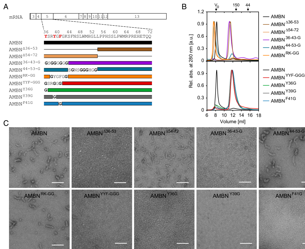
Fig. 1. Identification of residues essential for the self-assembly of AMBN. (A) Schematic representations of human Ambn mRNA, of the zoomed-out exon 5-encoded sequence comprising residues 36–72 of AMBN, and of the sequence modifications in the mutant AMBN variants. Letters in red represent residues identified as indispensable for AMBN self-assembly. The solid lines replacing the brown-colored bars represent the portions deleted in AMBN. The glycine residues indicated in bold represent the substitutions introduced into the original AMBN sequence. Amino acid numbering is based on the sequence of the mature AMBN protein lacking the secretion signal peptide (AMBN, sequence NP_057603.1). (B) Purified recombinant intact AMBN (black line) and its mutant variants (colored lines) were analyzed by SEC on a Superdex 200 10/300 column. The molecular masses of the globular protein standards are indicated in kilodaltons above the chromatograms. V_0 , void volume. (C) TEM of purified intact AMBN and of its mutant variants. (Primary magnification: 64,000 \times ). (Scale bars, 100 nm.)
