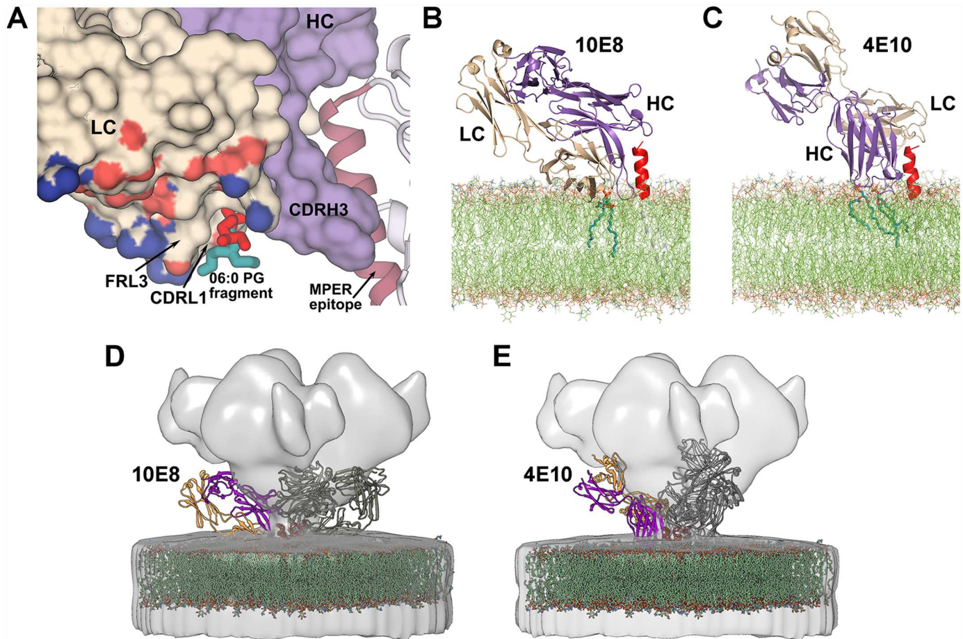
Fig 4. Integration of experimental data into a 10E8-MPER epitope-viral membrane model. (A) Surface rendering of the 10E8 Fab (beige, light chain; violet, heavy chain) showing the PG lipid fragment (red-dark cyan sticks) bound in a cavity formed between CDRL1, FRL3 and CDRH3 in the 10E8-T117v2-PG crystal structure. The helical 10E8 epitope residues in the T117v2 scaffold protein (gray) are shown in dark pink and the light-chain surface interacting with the viral membrane is colored by atom type. (B) Model of the 10E8 angle of approach with respect to MPER epitope-viral membrane during antibody engagement. (C) Model of the 4E10 angle of approach with respect to MPER epitope-viral membrane [23] for comparison. In both (B) and (C), the light and heavy chains are shown in beige and violet, respectively. The helical MPER epitope is shown in red and the lipid bilayer as thin green lines. The experimental bound lipids are shown as thicker dark cyan sticks in both structures. (D) and (E) Fitting our models of the viral membrane with 4E10 and 10E8 in the experimental EM map of the CD4-bound Env (EMDB-5455 [40]). The light and heavy chains are shown as yellow and blue cartoons. The lipid bilayers are shown in green and the MPER epitope as dark red helices.
