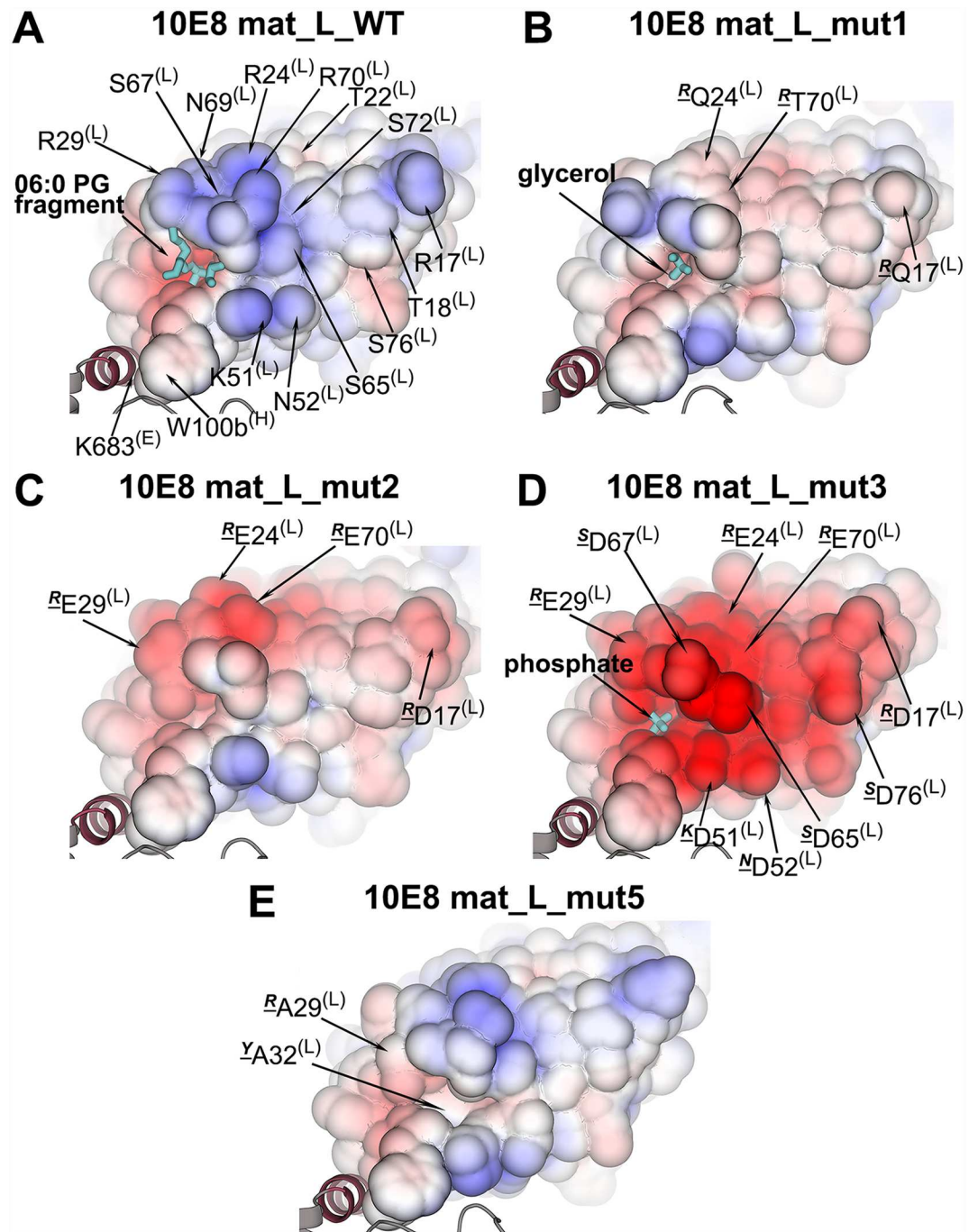
Fig 3. Distribution of charge on the surfaces of the 10E8 light-chain variants. The electrostatic solvent accessible surface (contoured at \pm 5 kT/e) of the light-chain region presumed to bind the viral membrane is shown for: (A) wild-type mature 10E8; (B) 10E8 mutant 1; (C) 10E8 mutant 2; (D) 10E8 mutant 3; (E) 10E8 mutant 5. Negative and positive charges are indicated in red and blue colored surfaces, respectively. The ligands bound in the lipid-binding site are shown as dark cyan sticks and the epitope scaffold is shown in gray. The underlined superscript letters designate the original residues in the 10E8 wild type.
