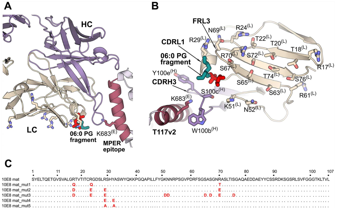
Fig 2. Design of 10E8 light-chain mutants. (A) Several light chain (LC; beige) basic residues (Arg and Lys shown as sticks) are in the same plane with the lipid head group (red and cyan sticks) and Lys683 (red sticks) of the gp41 MPER epitope (red). The heavy chain (HC) is shown in violet. (B) Light-chain surface residues (beige) that are presumed to face the viral membrane. The heavy-chain residues at the tip of CDRH3 are shown as violet sticks. The 10E8 peptide epitope (pink) from the T117v2 scaffold is shown up to Lys683 (pink; last residue of gp41 ectodomain). (C) Alignment of the amino-acid sequence of the five 10E8 light-chain mutants compared to wild-type 10E8. Only the variable region of the 10E8 light-chain variants are shown with the Kabat numbering scheme on top of the alignment. The mutations are highlighted in red.
