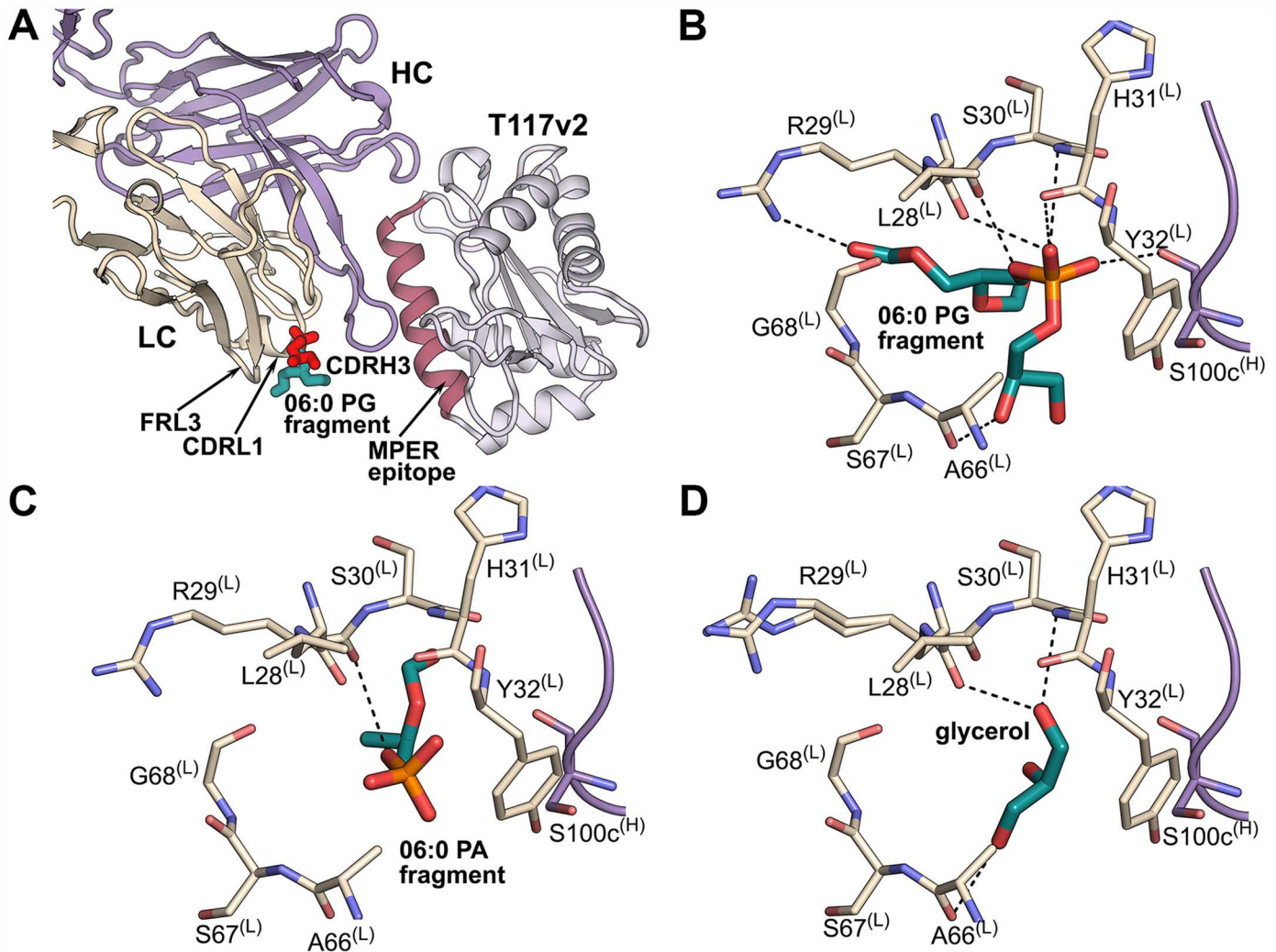
Fig 1. 10E8 lipid-binding site. (A) Crystal structure of the 10E8-T117v2 complex bound to 06:0 PG (sticks; red, glycerol and phosphate moieties of the head group; cyan, head group region linked to the lipid tails). The 10E8 light chain (LC) is shown in beige, heavy chain (HC) in violet, and T117v2 scaffold containing the MPER epitope (pink) in gray. This color scheme is used throughout. (B) All potential hydrogen-bond interactions (within ~3.5 Å) of the 06:0 PG fragment (colored by atoms) with 10E8 residues of CDRL1 (beige) and CDRH3 (violet) are shown as dashed lines. (C) All potential hydrogen-bond interactions (within ~3.5 Å) of the 06:0 PA fragment (colored by atoms) with CDRL1 (beige) and CDRH3 (violet) residues of 10E8. (D) All potential hydrogen-bond interactions (within ~3.5 Å) of a glycerol found in the lipid-binding site in the 10E8-T117v2 structure in the absence of added lipids.
