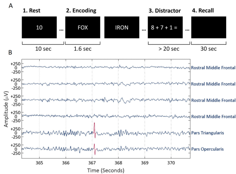
Figure 1. Study Design
