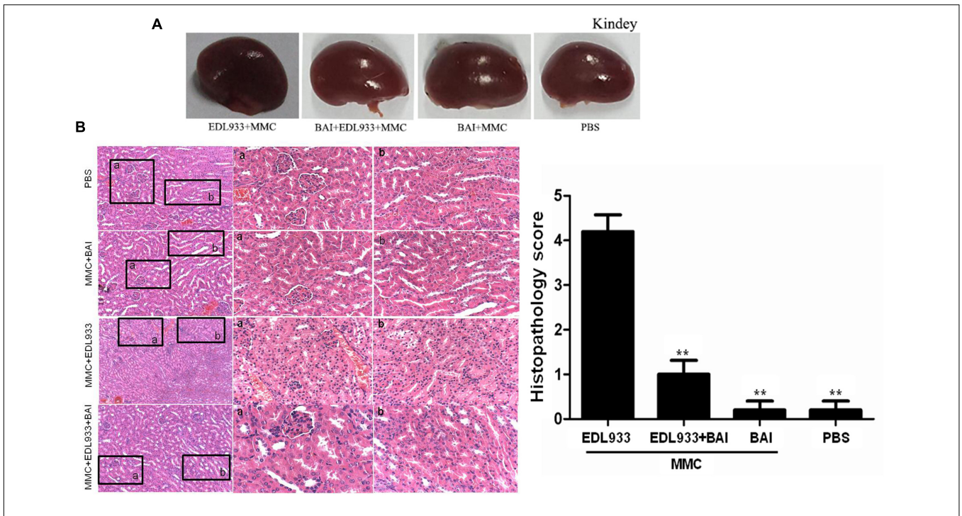
FIGURE 3 | Kidneys tissue and their histopathological examination by HE staining. (A) Comparison of kidneys tissue from differently treated mice. Note that kidneys from BAI-treated mice exhibited lower pathological abnormalities. (B) Histopathological examination of kidney tissue by HE staining. PBS and MMC+BAI group displayed standard kidney histopathology. a: complete glomerulus architecture, b: regular nuclear arrangement in renal tubule. EDL933 infection group space between the glomerulus and Bowman’s capsule; b: loss of brush border in the renal tubule, along with cytoplasmic attenuating and loss of the epithelial cells; loss of polarity of tubular cells and degeneration in the renal tubule. BAI administration improved kidney histopathology following EDL933 treatment. a: complete Bowman’s capsule and glomerulus architecture; b: renal tubule with distributed brush border; Regular nuclear arrangement, and well-development renal tubule. Histopathology scoring of renal glomerular degeneration and renal tubule necrosis by a veterinary pathologist: grade 0: no injury; grade 1: minimal injury with less than 10% of cells exhibiting degeneration or necrosis; grade 2: mild injury involving 10–25% of cells; grade 3: moderate injury involving 25–40% of cells; grade 4: marked injury involving 40–50% of cells; grade 5: severe injury involving greater than 50% of cells. N = 5, ** p < 0.01 vs. EDL933 infection group.
