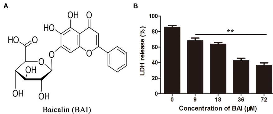
FIGURE 1 | Baicalin protects cells against toxins released by EHEC strain EDL933. (A) Chemical structure of Baicalin. (B) Inhibition of cell death by baicalin. Supernatant of EHEC EDL933 was added into Hela cells treated with indicated concentrations of baicalin for 36 h. Cell viability was evaluated by measuring extracellular LDH 36 h after adding the supernatant. All data represent the mean and standard error of three independent experiments. ** p < 0.01 .
