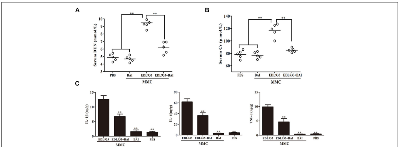
FIGURE 4 | Baicalin alleviated the pathologies induced by EDL933 infection. (A,B) The effects of baicalin on blood urea nitrogen (BUN) (A) and creatinine (Cr) (B) . Induced by EDL933 infection. The blood of relevant mice groups was evaluated for BUN and Cr at 6 days after treatment. Each circle represents the BUN or Cr level from one mouse, n = 5. (C) Baicalin reduced the production of several cytokines induced by EDL933. Kidney tissues from relevant mice were measured for cytokines by ELISA. Note the reduction of cytokine production in infected mice treated with baicalin. ** p < 0.01.
