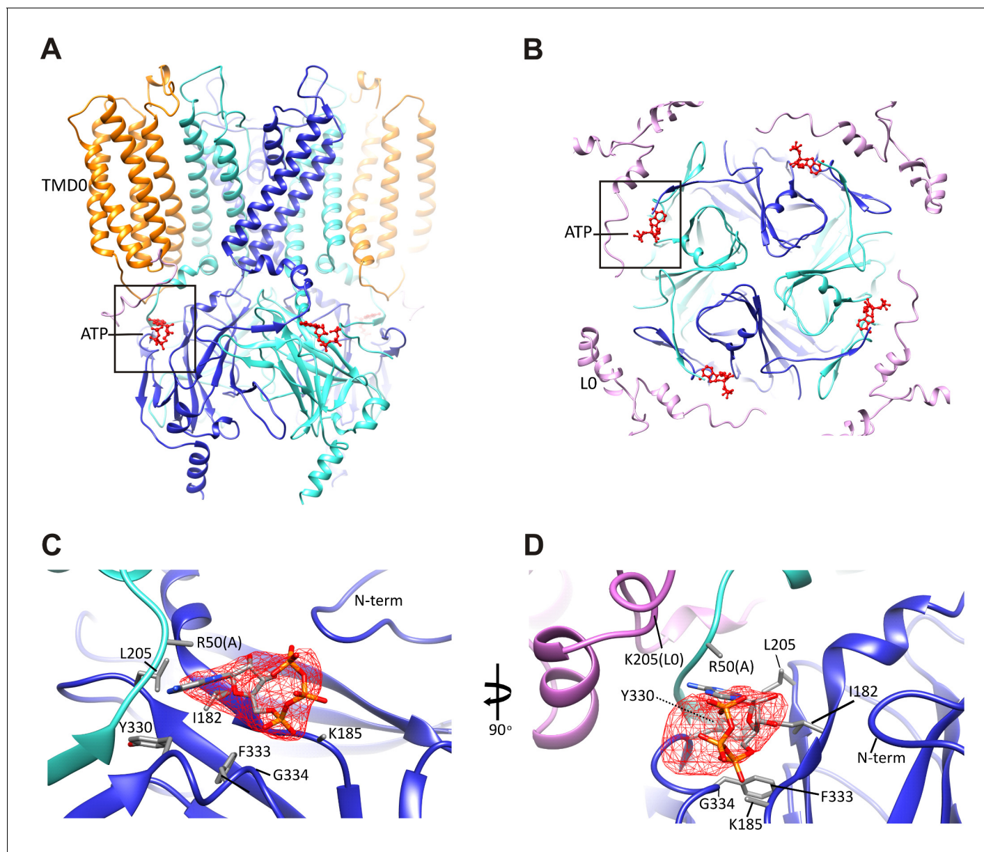
Figure 4. The ATP binding pocket. (A and B) Overview of ATP site from the side and from the top. (C and D) Difference map calculated from model prior to ATP docking, contoured to 3\sigma . Residues surrounding the ATP density are labeled. Side chains of residues with supporting density are shown. The N-terminus from Kir6.2 subunit A is colored in cyan and R50 is labeled followed by (A). The adjacent subunit is colored in blue, and SUR1-L0 is colored lavender, with the K205 position labeled.
