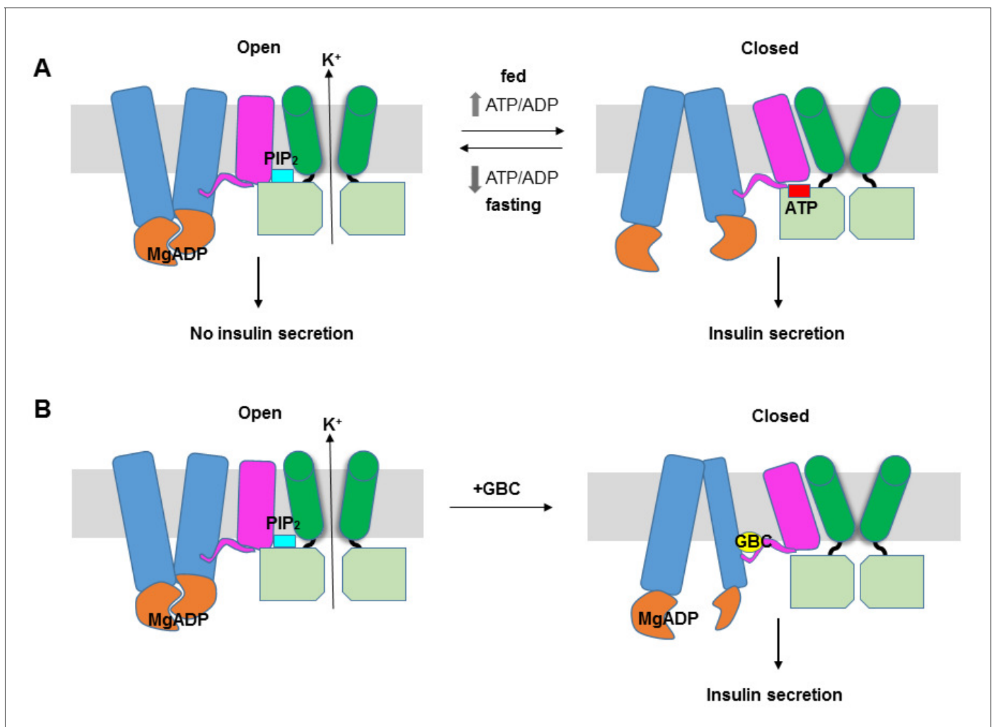
Figure 8. K_{ATP} channel gating model. (A) Cartoon illustrating how changes in the ATP/ADP ratio upon feeding and fasting alter the equilibrium between the inward-facing and outward-facing states of the SUR1-ABC core and interactions of the channel with ATP and PIP 2 to control channel activity. (B) Model of the hypothesized mechanism whereby GBC causes misalignment of the NBDs to prevent Mg-nucleotides activation of K_{ATP} channels. In both A and B, Kir6.2 transmembrane helices: green; Kir6.2 cytoplasmic domain: lime green; SUR1-TMD0/L0: magenta; SUR1-TMD1/2: blue; SUR1-NBDs: orange; GBC: yellow; ATP: red; PIP 2 : cerulean. Note the different states shown are not meant to reflect the actual conformational transitions.
