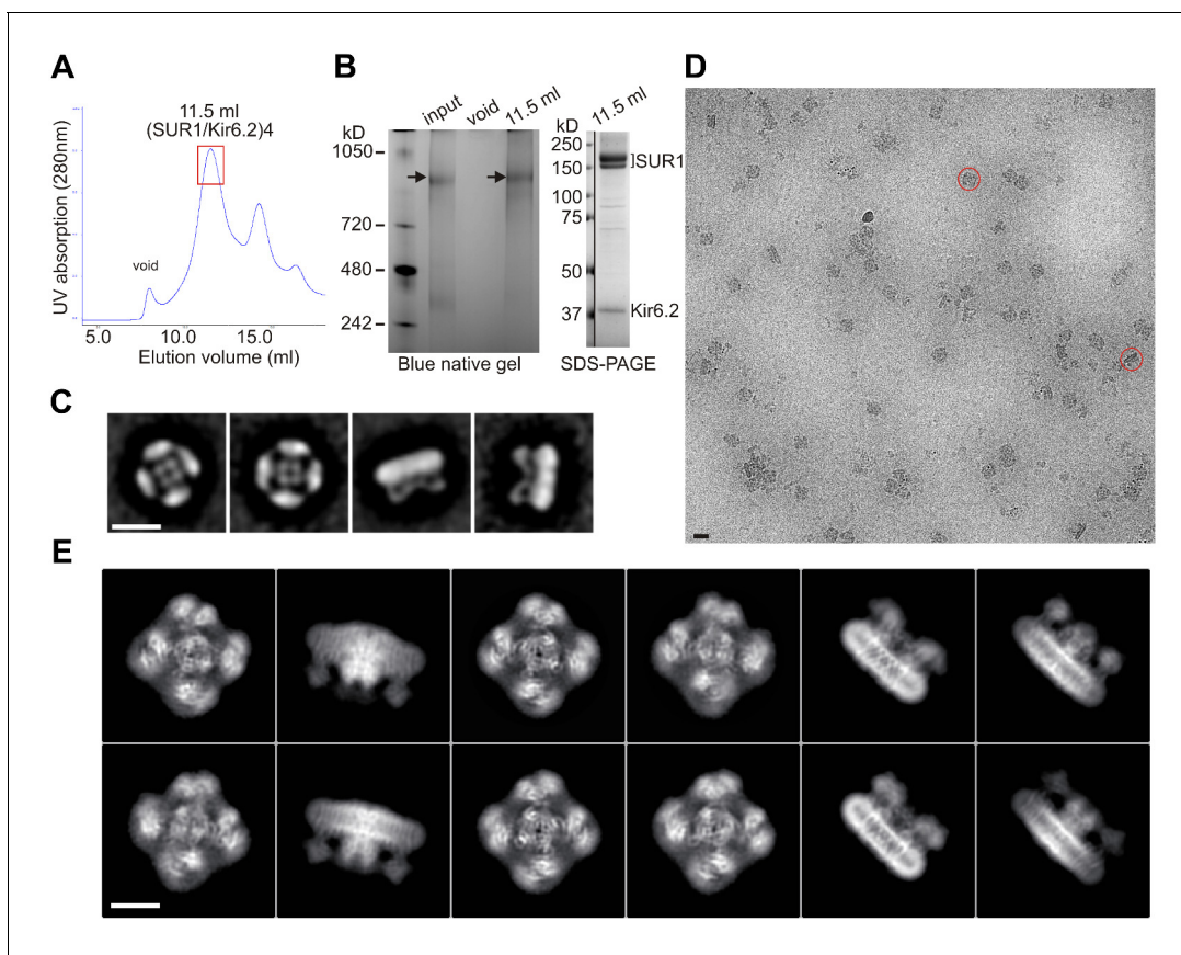
Figure 1. Purification and single-particle EM imaging of the SUR1/Kir6.2 K ATP channel. (A) Size exclusion chromatography (SEC) profile of affinity purified K ATP channels on a Suprose 6 column showing peak elution at ~11.5 ml (the red rectangle). (B) Left: Blue native gel showing the size of the purified complex at ~1 mDa (arrow) corresponding to four SUR1 and four Kir6.2. Input: samples eluted from anti-FLAG M2 agarose beads; void: sample from the SEC void fraction; 11.5 ml: sample from the SEC 11.5 ml elution fraction. Right: SDS-PAGE of the 11.5 ml fraction showing SUR1 (lower band: core-glycosylated; upper band: complex-glycosylated) and Kir6.2 as the main proteins. A vertical line separates MW markers from the sample lane in the same gel. (C) Negative-stain two-dimensional class averages showing topdown views (1, 2) and side views (3, 4) of the channel complex. (D) A representative cryoEM micrograph of K ATP channel particles imaged on an UltrAufoil grid. (E) Representative two-dimensional class averages of K ATP channels.
