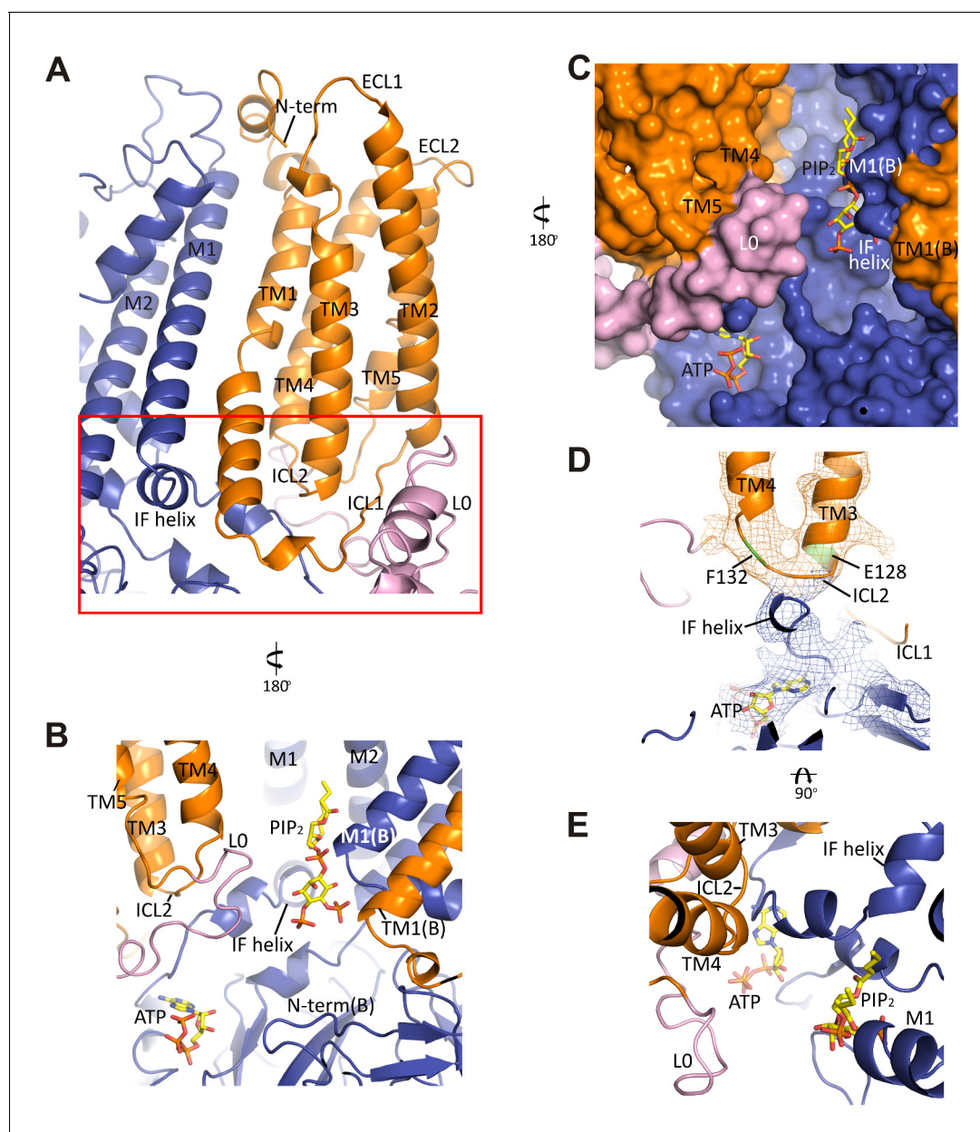
Figure 5. The interface between TMD0 and the N-terminal segment of L0 with Kir6.2. (A) Overall structure of the interface region, with TMD0 in orange, Kir6.2 in blue, and L0 in lavender. ECL: extracellular loop; ICL: intracellular loop; IF helix: interfacial (slide) helix. (B and C) Detailed view of the region boxed in red in (A) shown in ribbon (B) and surface (C) representations. ATP is docked as in Figure 3 and PIP 2 was docked hypothetically using PIP 2 bound Kir3.2 and Kir2.2 structures for placement. (D) A side view of the ICL2 showing close interactions with the Kir6.2 IF helix. E128 and F132, mutation of which alters channel P o and ATP sensitivity, are highlighted. (E) A top-down view of this region with both docked ATP (in the back) and PIP 2 in view.
