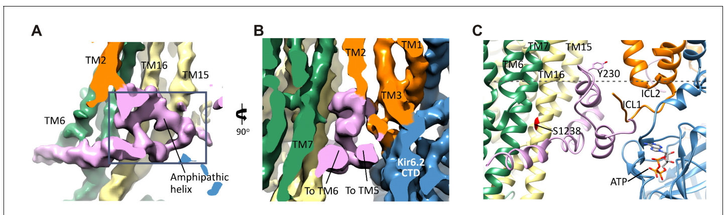
Figure 6. The SUR1-L0 connecting TMD0/Kir6.2 with the SUR1-ABC core. (A) View of the L0 region from the side along the plane of the membrane; Kir6.2 density has been removed for clarity. The hairpin structure is outlined. (B) Slice through the N- and C-terminal segments of L0. (C) Model of L0 highlighting relation between Y230 and S1238 (marked red) in TM16, which are separated by ~20 Å ( C\alpha to C\alpha ). Side chain of Y230 is shown based on supporting density. The gray dashed line marks the approximate boundary of the inner leaflet of the lipid bilayer.
