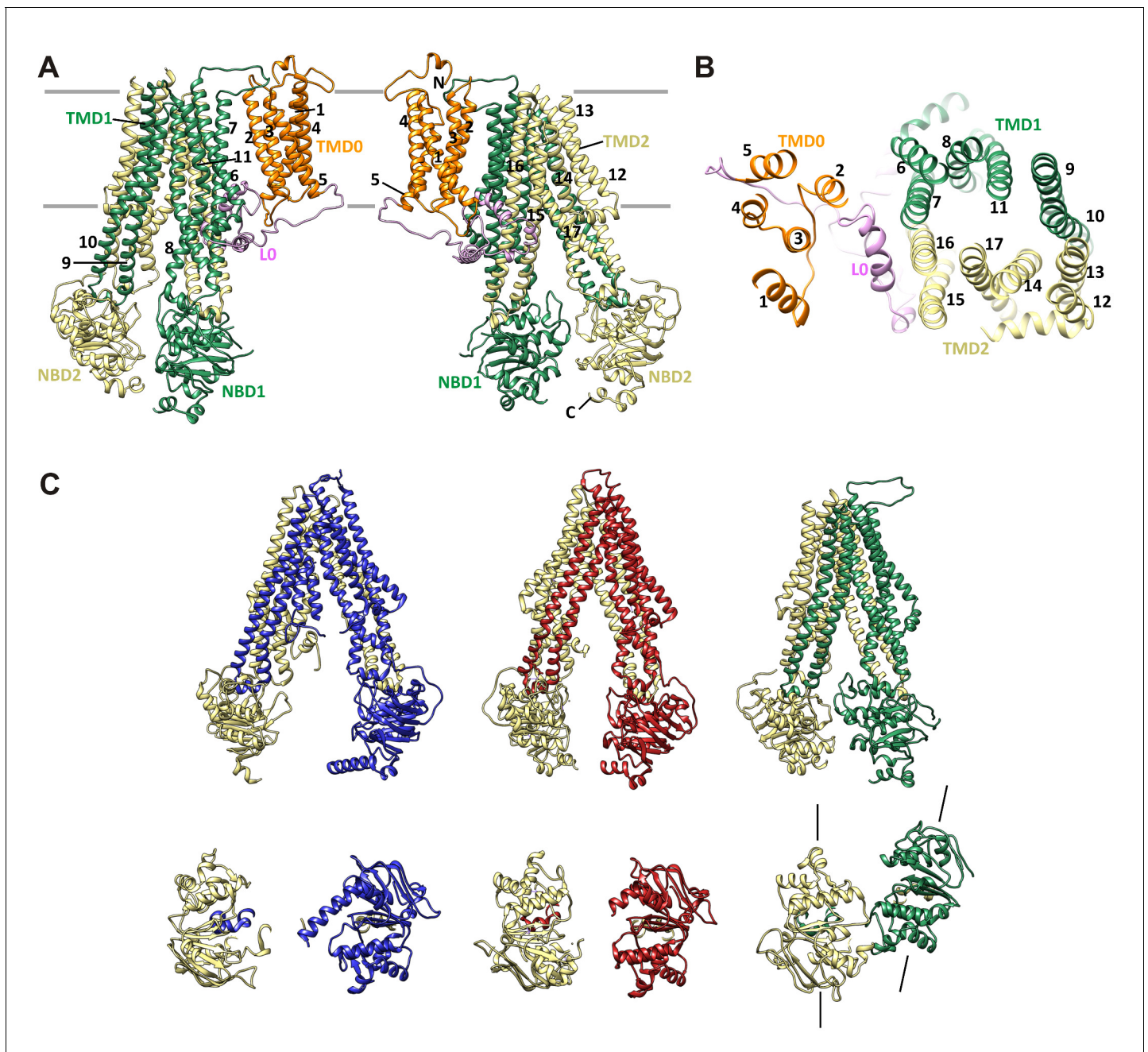
Figure 7. SUR1 with a twisted ABC core conformation in saturating concentrations of GBC. (A) Model of SUR1 with the various domains colored as in Figure 1 , with each TM helix labeled. On the left, TMD1/NBD1 (green) is toward the front and TMD2/NBD2 (tan) is toward the back. (B) Cross-section of the SUR1 model, showing relative orientation of each of the 17 TM helices and a helix in LO. (C) Comparison of inward-facing ABC transporter structures: From left, C. elegans Pgp (PDB code 4 F4C); mouse Pgp (4 M1M); hamSUR1. For each model, TMD2/NBD2 is colored tan. Lines on the side of the SUR1 NBDs denote the relative orientation of the NBD dimerization interface, demonstrating the observed twisting relative to other inward-facing structures.
