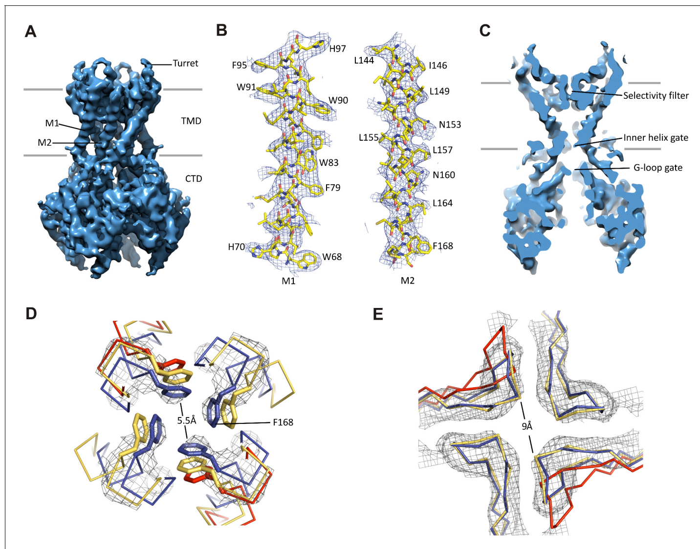
Figure 3. Kir6.2 in a closed conformation. (A) Cryo-EM density map of Kir6.2 at 5.1 Å resolution. (B) Density of M1 and M2. Residues with clear side chain density are labeled. (C) A central slice through the density highlighting the ion permeation pathway. (D) View of the inner helix gate (F168) looking down the pore from the extracellular side. Kir3.2 apo (yellow, PDB ID: 3SYO) and Kir3.2-R201A+PIP 2 (red, 3SYQ) structures were aligned to the region surrounding the gate. (E) Comparison of G-loop conformations of Kir6.2 and Kir3.2 (3SYO and 3SYQ) by alignment of the cytoplasmic domain; same coloring as in (D). The distance shown in (D) and (E) is between the main chains; the constriction should be even narrower due to side chains that should be protruding into the pore, as is seen in homologous structures. Density depictions contoured to 2.5σ in (B, D, E).
