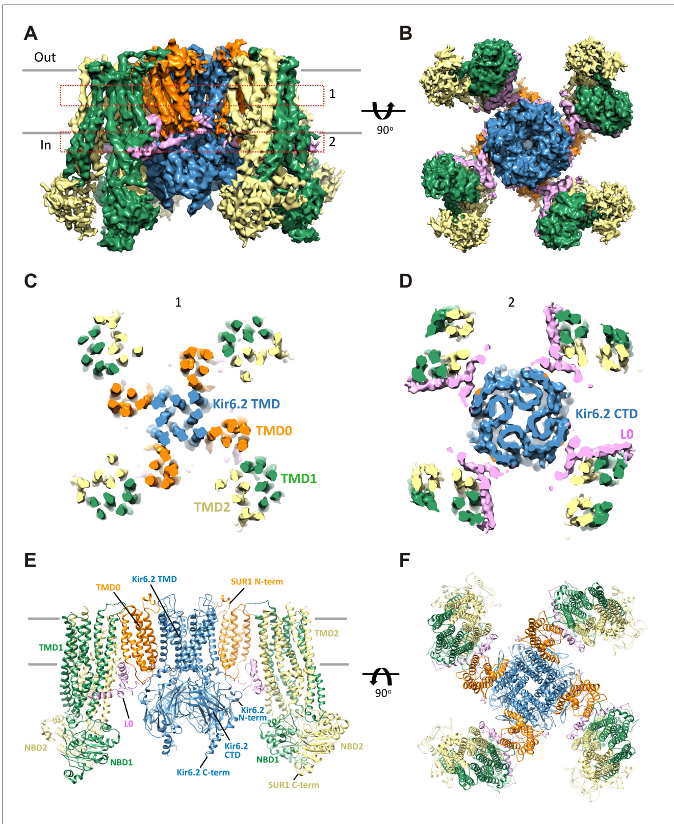
Figure 2. Three-dimensional reconstruction of the K_{ATP} channel. (A) Cryo-EM density map of the K_{ATP} channel complex at an overall resolution of 5.8 Å, viewed from the side. The four Kir6.2 subunits in the center are colored blue, SUR1 is in orange (TMD0), lavender (LO), green (TMD1/NBD1), and yellow (TMD2/NBD2). Gray bars indicate approximate positions of the lipid bilayer. (B) View of the complex from the cytoplasmic side. (C and D) Cross-section 1 and 2 of the complex. (E) Ribbon diagram of the complex. (F) Ribbon diagram of the complex from the cytoplasmic side. Figure 2 continued on next page
