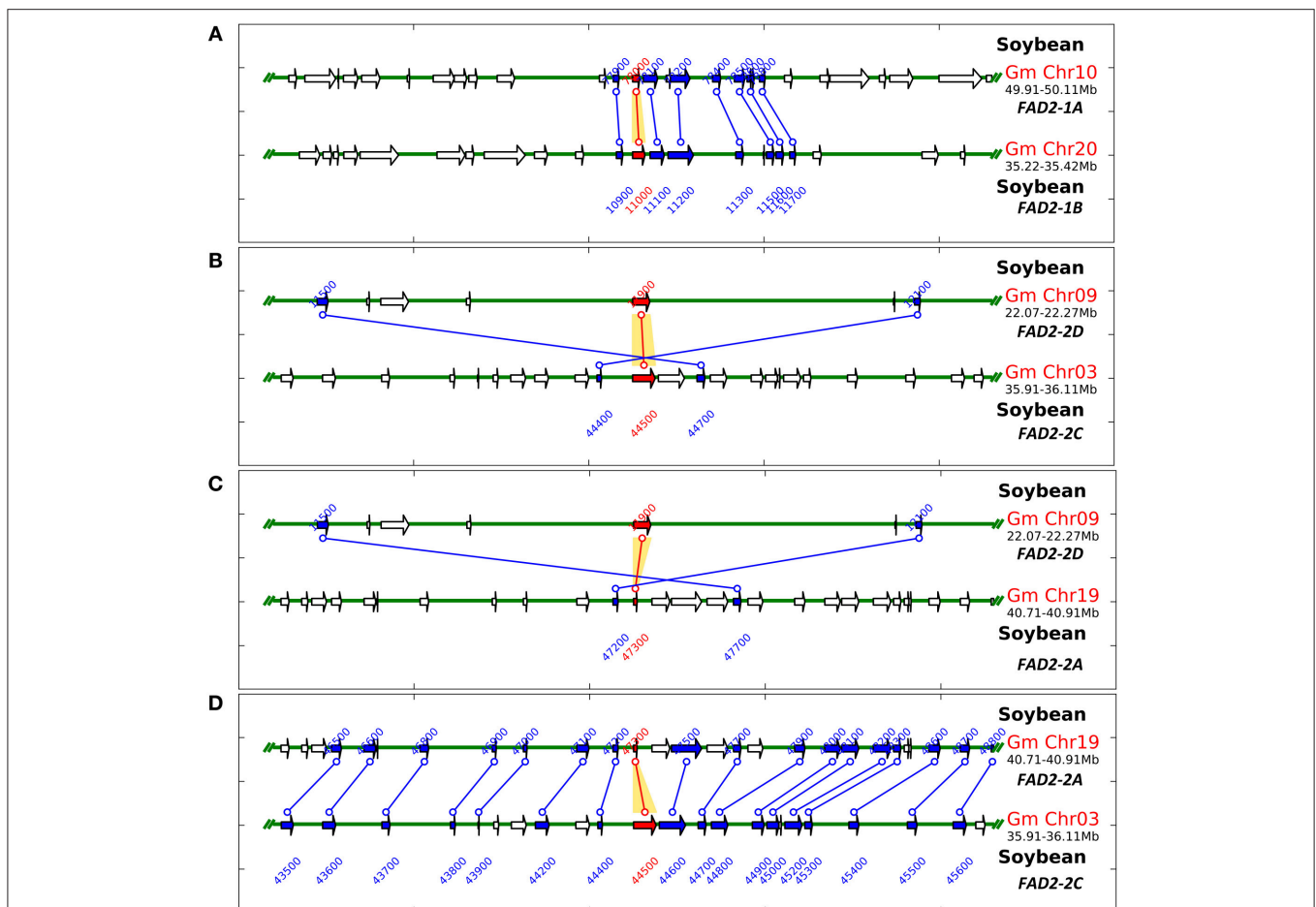
FIGURE 1 | Schematic representation of GmFAD2 containing duplicated segments identified in the soybean genome. Soybean FAD2 intragenome syntenic relationships were calculated using the Plant Genome Duplication Database ( http://chibba.agtec.uga.edu/duplication/ ). (A) GmFAD2 in chr10 and chr20 belongs to another duplicated segment with less conserved genes; just 8 duplicated genes or anchors. (B) GmFAD2 in chr03 and chr09 belongs to a third duplicated segment containing 19 additional inverted duplicated genes or anchors. (C) GmFAD2 in chr19 and chr09 belongs to a third duplicated segment containing 21 additional inverted duplicated genes or anchors. (D) GmFAD2 in chr19 and chr03 belongs to a very large duplicated segment containing 1,060 additional conserved duplicated genes or anchors. Graphs represent \pm 100 kb duplicated region centered in the GmFAD2 gene.
