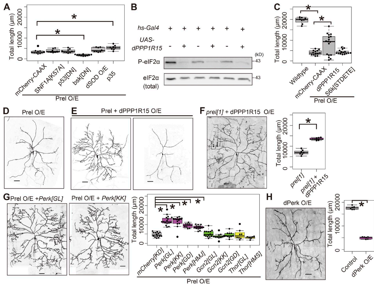
Figure 4. Promotion of eIF2 \alpha dephosphorylation prevents the dendritic loss induced by prel O/E. (A) The effect of repression of candidate pathways of mitochondria-derived stress signaling on the dendritic loss induced by Prel O/E in class IV neurons. bsk[DN] , a dominant-negative form of JNK; p53[DN] , a dominant-negative form of p53; SNF1A[K57A] , a kinase inactive form of AMPK catalytic subunit (Adachi-Yamada et al., 1999; Ollmann et al., 2000; Johnson et al., 2010). Expression of p35 , the baculovirus-derived inhibitory protein of effector caspases, slightly restored dendritic length of Prel-overexpressing class IV neurons (Hay et al., 1994). However, the degree of recovery was not striking, indicating a minor role of caspase activation in the dendritic loss. Analysis of variance (ANOVA) followed by post-hoc Dunnett's test (versus mCherry-CAAX ). (B) Immunoblot analysis revealed promotion of eIF2 \alpha dephosphorylation by dPPP1R15 O/E. dPPP1R15 was overexpressed using hs-Gal4 , which drives Gal4 expression by a heat-inducible Hsp70 promoter. Whole larvae treated with a heat shock (37°C for 1 h) were lysed 10 h after the treatment. Lysates were immunoblotted with anti-phosphorylated eIF2 \alpha (P-eIF2 \alpha ) and anti-eIF2 \alpha antibodies. Results of three biological replicates are shown. (C–G) Genetic interactions between O/E or loss-of-function of prel and eIF2 \alpha phosphorylation-related genes. Quantification of the effects of coexpression of dPPP1R15, S6k[STDETE], and mCherry-CAAX (UAS copy number control) with Prel on the dendritic length of class IV neurons (C). Note that the values of the total dendritic length of neurons that expressed dPPP1R15 and Prel were apparently distributed in a bimodal fashion (see also E). S6k[STDETE]: an active form of S6k (Barcelo and Stewart, 2002). ANOVA followed by post-hoc Dunnett's test (versus mCherry-CAAX ). Representative images of the dendritic arbors of Class IV neurons expressing Prel plus mCherry-CAAX (D) or dPPP1R15 (E; see also Fig. S4 A). An example of dendritic arbors (F, left) and quantification of the total dendritic length (F, right) of prel mutant class IV MAR CM clones overexpressing dPPP1R15. Representative images (G, left) and quantification of the total dendritic length (G, right) of class IV neurons with Prel O/E plus KD of Perk , Gcn2 , or Thor/4EBP . The amplicon for RNAi of Perk[HMJ] line does not overlap with those of other RNAi lines. ANOVA followed by post-hoc Dunnett's test (versus mCherry[KD] ). (H) Representative images (left) and quantification of the total dendritic length (right) of dPerk-overexpressing class IV neurons. *, P < 0.05 . Bars, 50 \mu m.
