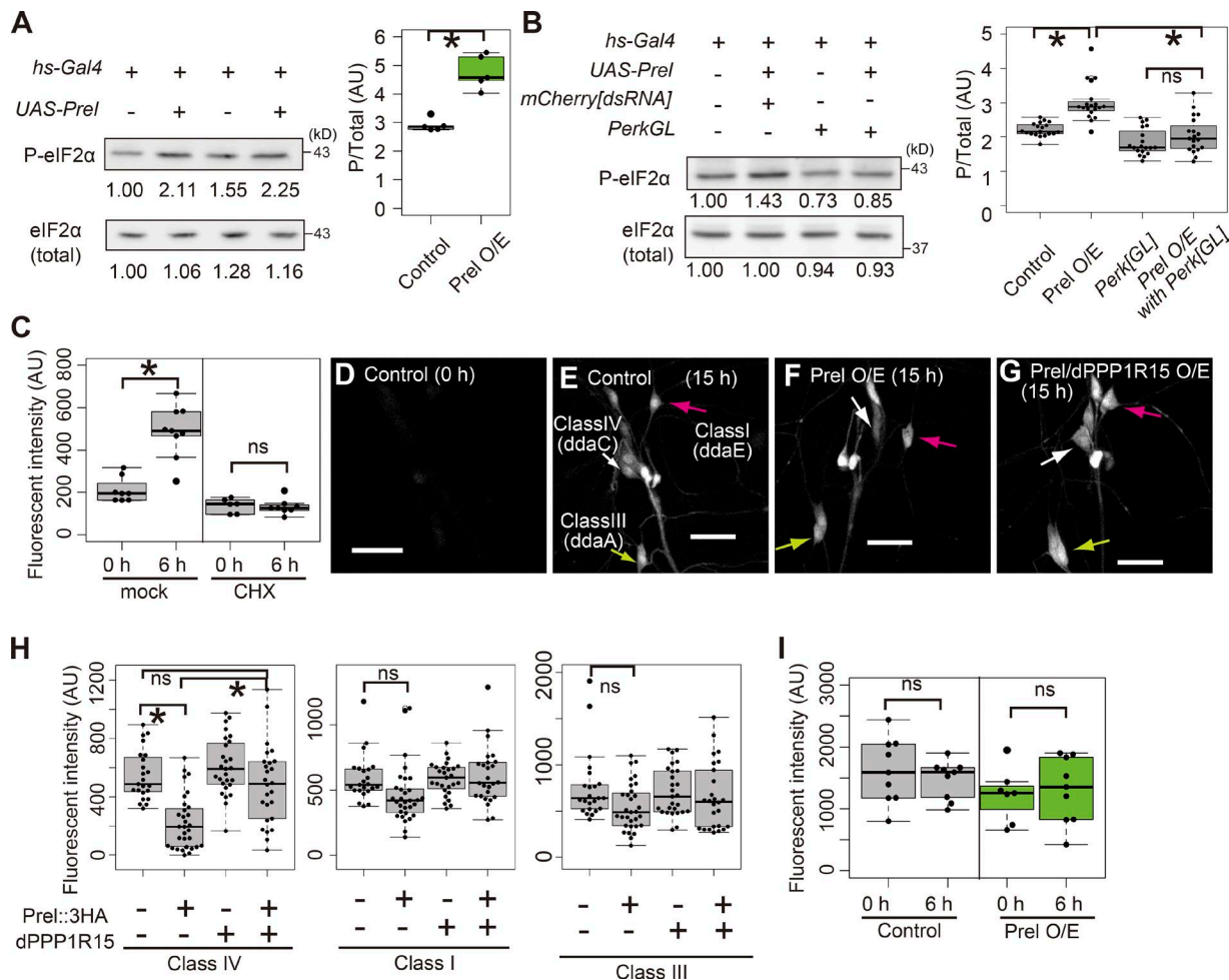
Figure 5. Differential eIF2 \alpha phosphorylation-mediated translational repression in da neurons. (A) Prel O/E increased P-eIF2 \alpha in vivo. Prel was overexpressed by using hs-Gal4 . Brain lysates of control and Prel-overexpressing adult female flies treated with heat shocks were immunoblotted using antibodies against P-eIF2 \alpha or total eIF2 \alpha . Immunoblots of two biological replicates are shown and relative values of band intensities are indicated (left). Quantification of the band densities of five biological replicates (right). (B) The increase in the P-eIF2 \alpha amount by Prel O/E was partially suppressed by KD of Perk ( Perk[GL] ). A representative immunoblot of brain lysates and relative values of band intensities (left). Quantification of the band densities of 19 biological replicates (right). (C) Kaede imaging in da neurons detected translational repression induced by cycloheximide (CHX), an inhibitor of protein translation. Early L3 larvae expressing Kaede in da neurons were prefed with a fly food containing CHX for 4 h before photoconversion (PC). Whole larvae were irradiated with UV light. Intensity of unconverted, green Kaede fluorescence in the soma was quantified. Half of the photoconverted larvae were observed immediately after PC (0 h), and the other half were aged in the fly food containing CHX for 6 h, then observed (6 h). AU, arbitrary units. (D–H) Prel O/E preferentially suppressed representative protein synthesis in class IV neurons. Grayscale images of unconverted Kaede fluorescence in control (D and E), Prel O/E (F), and Prel plus dPPP1R15 coexpression (G). Whole early L3 larvae were irradiated with UV light and aged for 15 h. Arrows indicate the soma of class IV (white), class I (magenta), and class III (yellow) neurons. Bars, 50 \mu m. Quantification of unconverted Kaede signals in the soma of da neurons (H). Unconverted Kaede signals immediately after and 15 h after PC were quantified. ANOVA with the post-hoc Tukey-Kramer method. (I) Quantification of the intensity of photoconverted Kaede just after conversion (0 h) and 6 h after conversion (6 h) in class IV neurons of either control or Prel O/E. *, P < 0.05 ; ns, not significant.
