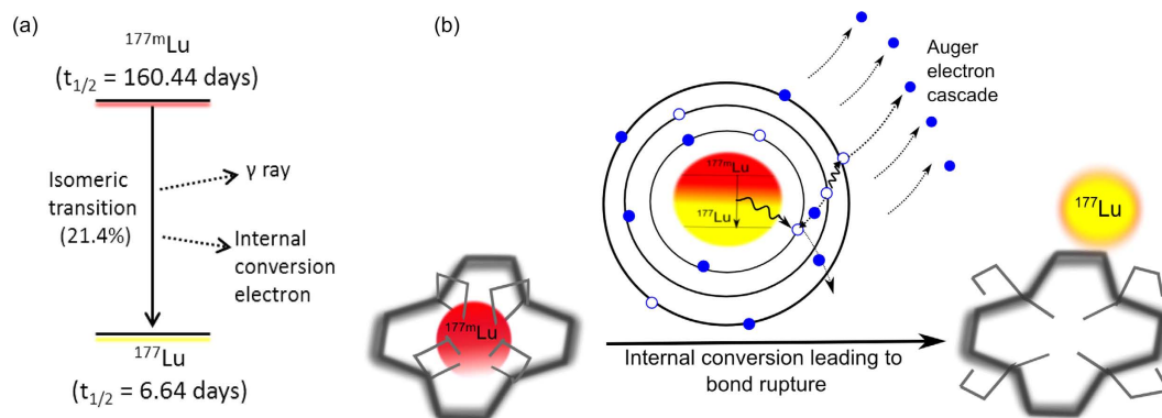
Figure 1. Schematic representation of the decay process. (a) Decay scheme of ^{177m}\text{Lu} to ^{177}\text{Lu} . (ii) Process of bond rupture. The metastable isomer ^{177m}\text{Lu} is coordinated to a very stable complex (left side). During the decay via internal conversion the nucleus excess of energy is transferred to an inner electron causing an Auger electron cascade (center). After the cascade the atom is in a highly charge state, the chemical bonds are broken and the freed ^{177}\text{Lu} can be separated (right side).
