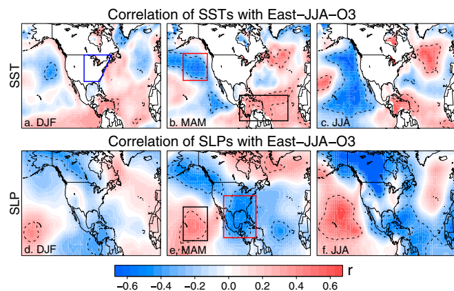
Fig. 1. Correlations of mean JJA MDA8 ozone in the eastern United States (East-JJA-O 3 ) with seasonal mean SSTs ( A–C ) and SLPs ( D–F ) for the seasons leading up to and including summer for 1980–2013. The blue quadrangle in A indicates the domain of East-JJA-O 3 . The dashed contour lines enclose regions in which the correlations reach statistical significance ( P < 0.05 ). We define the MAM- \Delta SST index as the average difference in MAM SSTs between the northern tropical Atlantic ocean (black rectangle in B ) and the northeastern Pacific ocean (red rectangle) and the MAM- \Delta SLP index as the average difference in MAM SLP between the eastern Pacific (black rectangle in B ) and a large region including much of the eastern and central United States, Mexico, and the Gulf of Mexico (red rectangle). SSTs are from ERSST v3b. Meteorological data are from NCEP. Ozone data are from the EPA Air Quality System. All data are detrended by subtracting the 7-y MAs.
