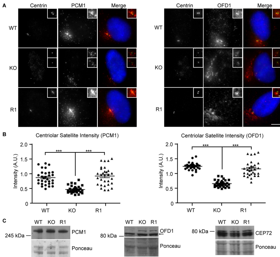
FIGURE 5: Reduced centriolar satellite density in C-NAP1-knockout cells. (A) Immunofluorescence microscopy of the indicated satellite markers in cells of the indicated C-NAP1 genotype. Scale bar, 5 μm. (B) Quantitation of the centriolar satellite density in cells of the indicated genotype. Maximum intensity projections of 10 centrosomes from G1 cells were analyzed in three separate experiments. Graphs show the sum of PCM1 or OFD1 fluorescence intensities in a 25-μm 2 circle around the two centrioles in each cell in arbitrary fluorescence units (A.U.). (C) Immunoblot of centriolar satellite proteins in cells of the indicated genotype. Ponceau S staining of the membrane after protein transfer was used as a loading control. *** p < 0.001 by unpaired t test.
