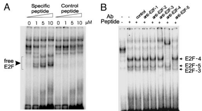
Fig. 4. Effect of cell-penetrating interfering peptide on free E2F levels. (A) In DNA gel-shift assays using ^{32} P-labeled E2F oligonucleotide and nuclear extracts from adipocytes, cell-penetrating peptide (specific and control peptides) was added to binding reactions at increasing concentrations. (B) Nuclear extracts (day 8) were preincubated with the cell-penetrating interfering peptide together with specific antibodies against different E2F members for 15 min and then analyzed for E2F DNA-binding activity by gel-shift assays as above.
