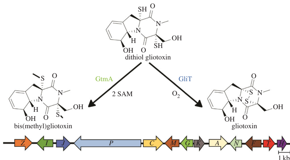
Figure 1. Conversion of gliotoxin between the reduced (dithiol gliotoxin), oxidized (gliotoxin) and bishthiomethyl forms. In A. fumigatus , the gli -cluster that encodes gliotoxin biosynthesis consists of 13 genes (in colour and labelled with their last letter) and is located on chromosome 6 [4–6]. gtmA is encoded outside the cluster and is on chromosome 2.
