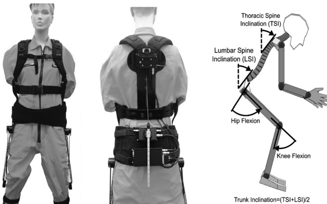
Fig. 2. Front and back view of the CUELA measuring system and stick figure to demonstrate the outcome parameters for gait (Note: the direction of the arrows shows the positive direction of the outcome parameter)
