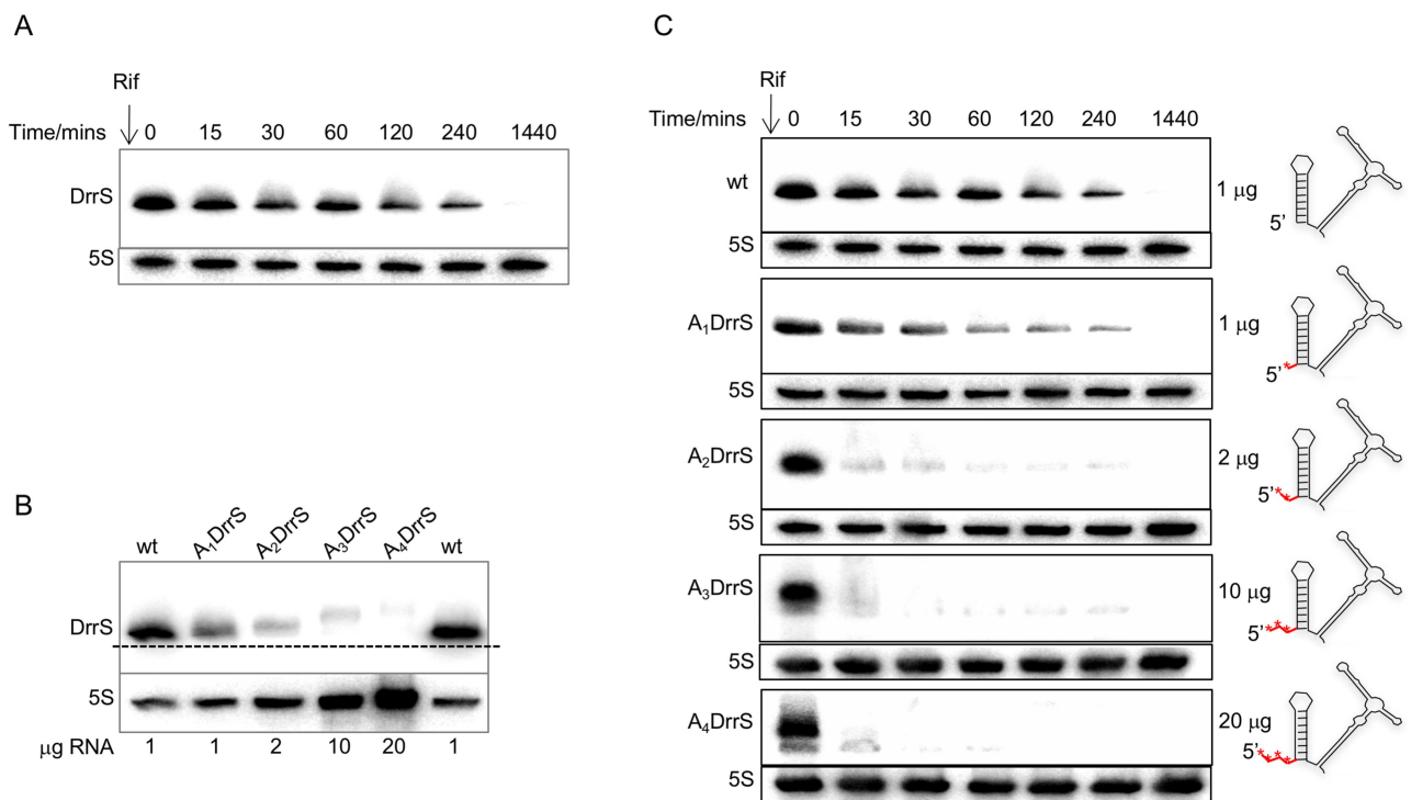
Fig 9. Turnover of DrrS and its 5' derivatives in M. smegmatis . A: Northern blot of total RNA from M. smegmatis expressing DrrS from a heterologous promoter. Rifampicin (200 μg/ml rifampicin) was added at time zero and RNA was isolated at the indicated time point and probed for DrrS as previously described. B: Northern blot of 1–20 μg of total RNA from M. smegmatis expressing wildtype and 5' variants of DrrS. RNA from the strain expressing wildtype DrrS was loaded in the first and last wells to ensure proper alignment. C: Turnover of DrrS 5' variants. Each DrrS 5' variant was expressed in M. smegmatis , cultures were grown to OD 600 = 0.6 and rifampicin added to a final concentration of 200 μg/ml. Samples were withdrawn at the indicated time points and subjected to Northern blotting. As the relative amount of DrrS varied significantly between the wildtype and the derivatives (see panel B), different amounts of total RNA were loaded on the gels, i.e. 1 μg each wildtype and A 1 DrrS; 2 μg of A 2 DrrS; 10 μg A 3 DrrS and 20 μg A 4 DrrS. Cartoon on the right illustrate the 5' additions (red asterisks) to the DrrS structure.
