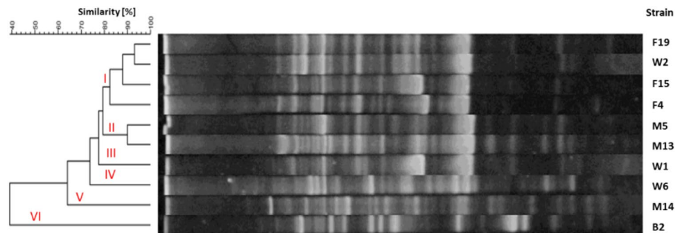
Fig. 4 Dendrogram derived from RAPD-PCR profiles of Staphylococcus xylosus generated with the Xyl2 primer. F isolates from bioaerosol, M isolates from masks, W isolates from swab, B isolates from biomass
