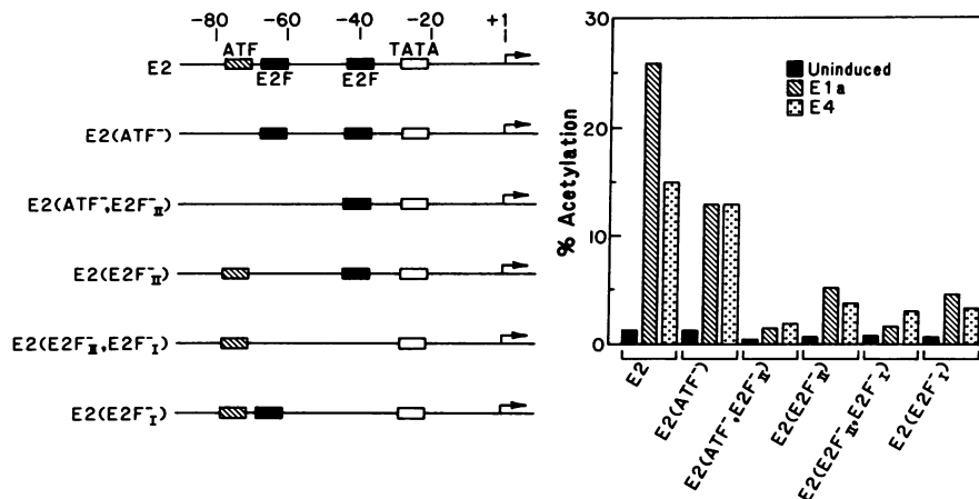
FIG. 1. E2 promoter requirements for E1A - and E4 -mediated trans-activation. (Left) Schematic diagram of the E2 promoter substitution mutants as described by Loeken and Brady (9). (Right) Results of trans-activation assays with the various E2 promoter mutants. Vero cells were transfected with 10 \mu g of the E2 promoter-CAT constructs either alone or together with pE1A (10 \mu g) or pE4 (10 \mu g). Cells were harvested for CAT assays as described. CAT activity was quantitated by scintillation counting of appropriate regions of the TLC plate.
