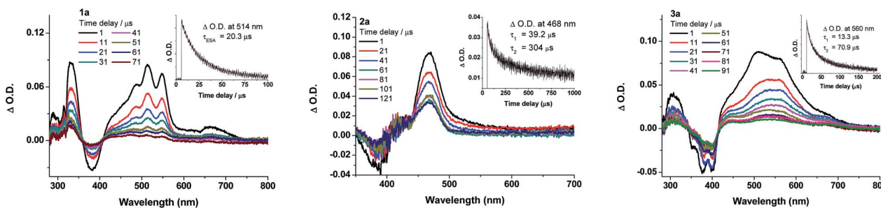
Fig. 7 Nanosecond transient absorption (ns-TA) difference spectra of 1a–3a (5 recorded at selected decay times in degassed \text{CH}_2\text{Cl}_2 ( 5 \times 10^{-5} M) at 298 K. Insets show the ESA kinetic decay trace at the specified wavelengths; decay lifetimes were fitted as mono-exponential decay for 1a and bi-exponential decays for 2a and 3a . ( \lambda_{\text{exc}} = 355 nm; integration time: 200 ns).
