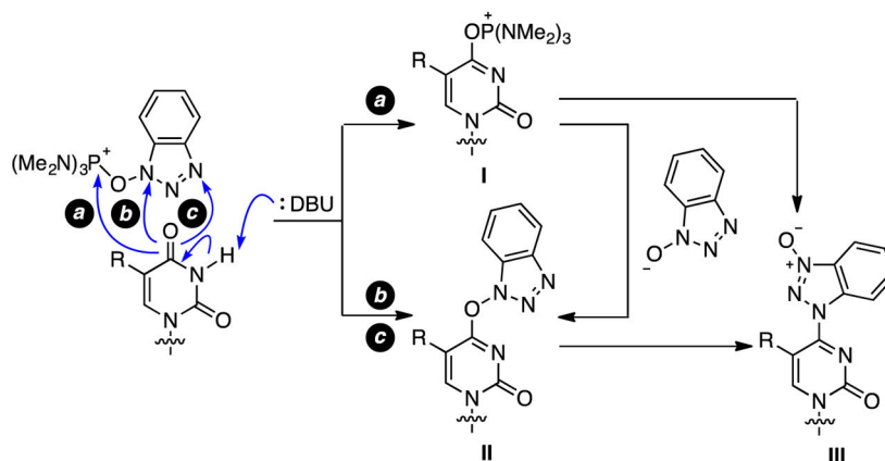
Scheme 1. Some mechanistic considerations.
