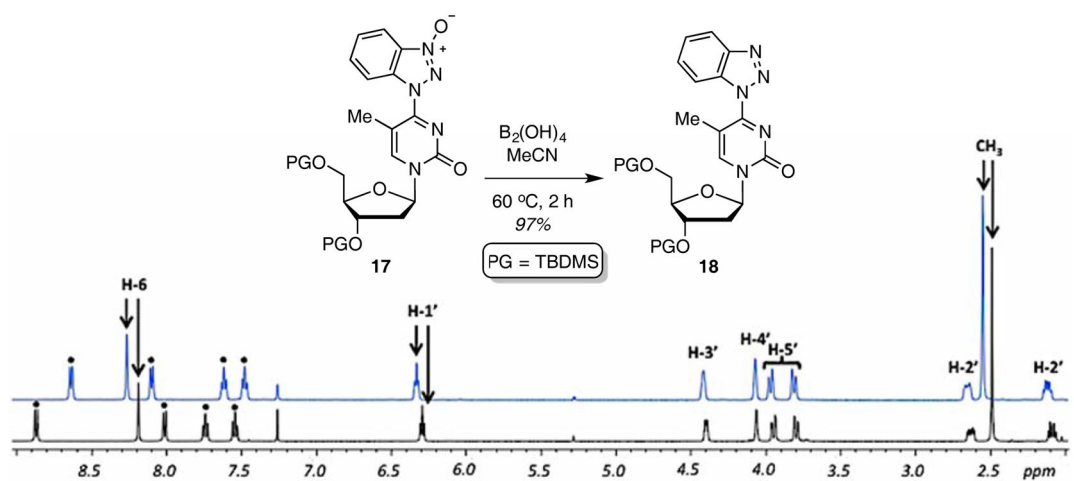
Fig. 3. Partial NMR spectra of compounds 17 (in black) and 18 (in blue) in CDCl_3 . Benzotriazolyl resonances are indicated by dots and TBDMS resonances are not shown.
