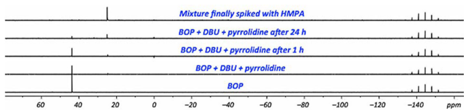
Fig. 5. ^{31}\text{P}\{^1\text{H}\} NMR spectra in \text{CD}_3\text{CN} to observe for changes when BOP is in contact with DBU and pyrrolidine at room temperature.
