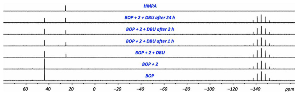
Fig. 4. ^{31}\text{P}\{^1\text{H}\} NMR spectra in \text{CD}_3\text{CN} to observe for changes during the course of the reaction at room temperature.
