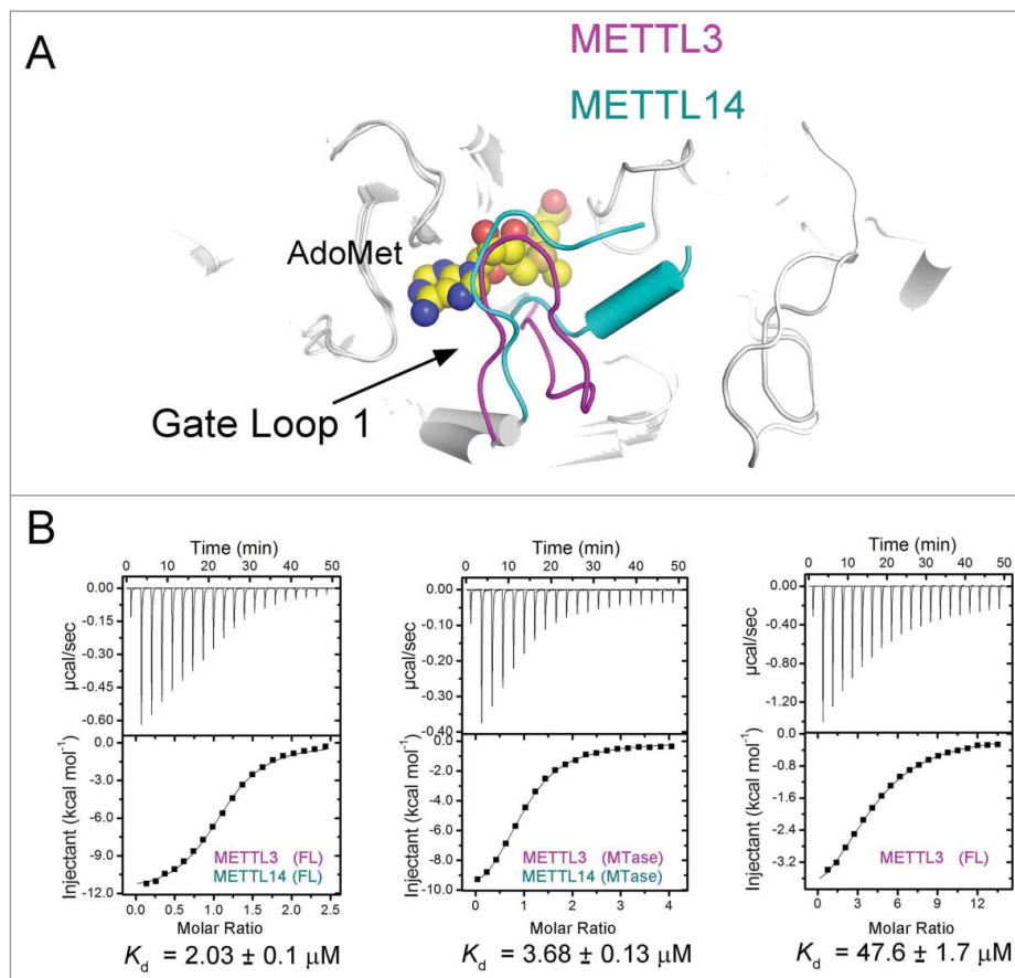
Figure 2. (A) Superposition of AdoMet-bound METTL3 and METTL14. AdoMet is shown in space-filling view. Gate loop 1 in METTL3 and METTL14 is colored in magenta and cyan, respectively. (B) Measurement of binding affinity between AdoMet and the METTL3-METTL14 complex using ITC. The first data point was removed from the analysis. The dissociation constant ( K_d ) of the wild type was approximately 2.0 \mu\text{M} . The AdoMet binding affinity of the methyltransferase domain complex was comparable to wild type. METTL3 alone exhibited significantly reduced AdoMet binding activity.
