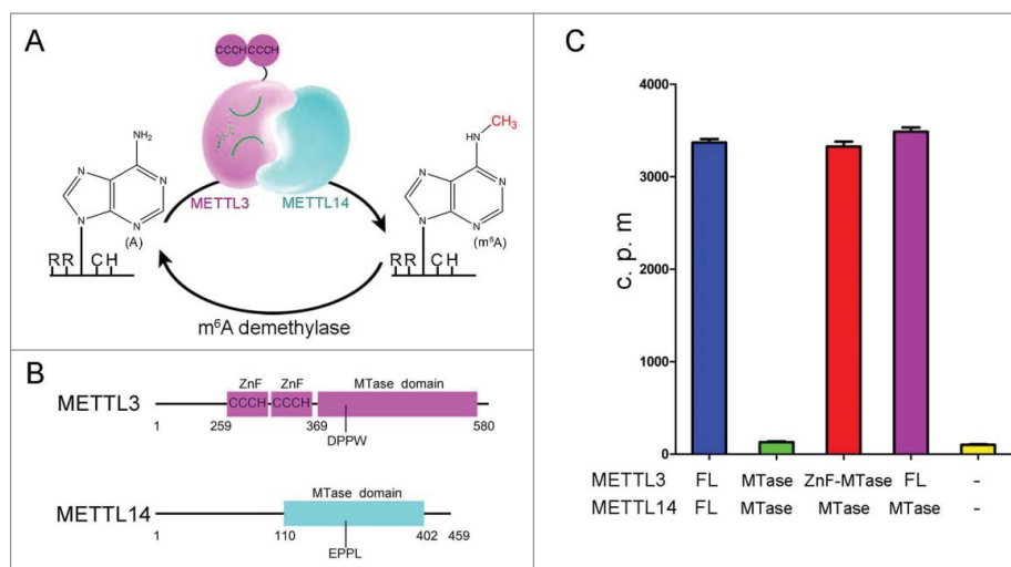
Figure 1. (A) Proposed model for reversible m^6A methylation. m^6A on RRACH is mainly appended by the METTL3-METTL14 complex, and oxidative demethylation is performed by m^6A demethylase. CCCH: Cys-Cys-Cys-His type zinc finger motif (ZnF). (B) Schematic illustration of METTL3 and METTL14 domain structures. The METTL3 ZnF and METTL3 methyltransferase (abbreviation as MTase) domains are colored in magenta, and the METTL14 methyltransferase domain is colored in cyan. Detailed domain boundaries are labeled beneath the structures. (C) Comparison of the methyltransferase activity of full-length (abbreviation as FL) and truncated methyltransferase complexes. The c.p.m. of the extracted RNA was measured in a scintillation counter and averaged ( \pm s.e.m.); the c.p.m. was determined from 3 replicates.
