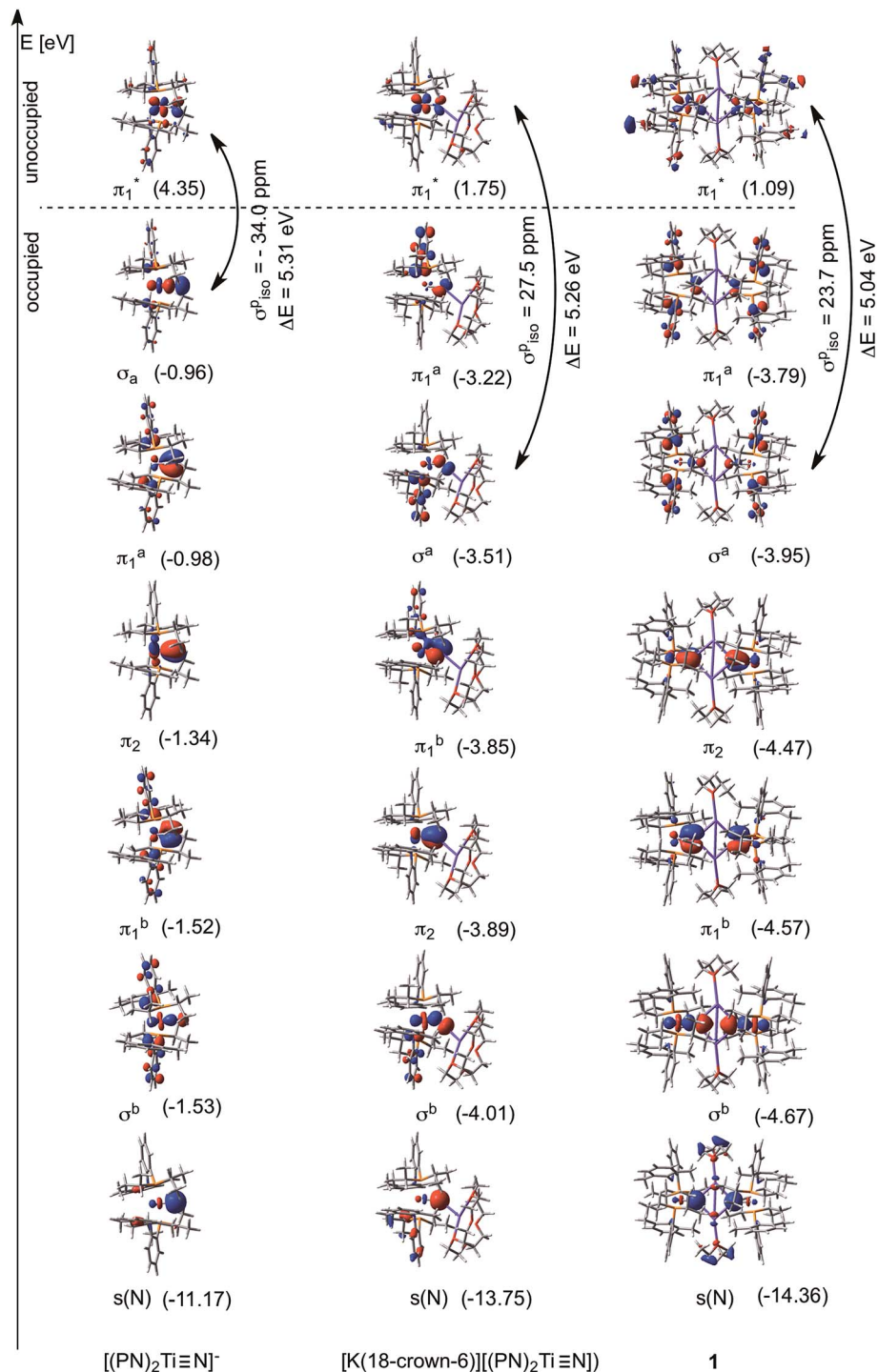
Fig. 10 Most relevant occupied MOs for [(\text{PN})_2\text{Ti}\equiv\text{N}]^- , [\text{K}(\text{18-crown-6})][(\text{PN})_2\text{Ti}\equiv\text{N}] and 1 describing the electronic structure of the \text{Ti}\equiv\text{N} functionality. One of the unoccupied orbitals, \pi_1^* , which is critical for the paramagnetic shielding of \text{N}_{\text{nitride}} is also depicted.
