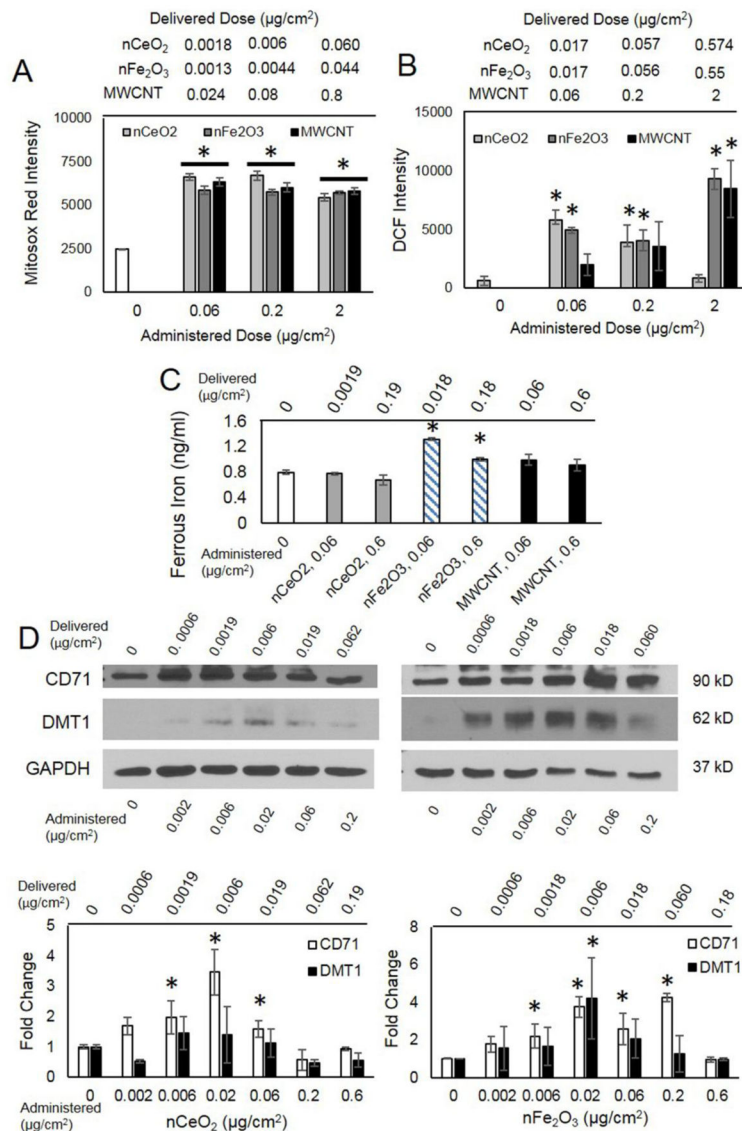
Figure 5. ROS generation and iron homeostasis disruption in nFe 2 O 3 -exposed SAECs. A) Superoxide production at 1 h (Mitosox Red) and B) ROS levels (DCF) intensity quantification after 24 h exposure in pSAECs. C) Ferrous iron intracellular concentrations following acute 24 h exposure in SAEC-hTERT. D) Enhanced transferrin receptor (CD71) and divalent metal transporter 1 (DMT1) expression following 24 h acute exposure to nCeO 2 and nFe 2 O 3 in SAEC-hTERTs. MWCNT dosimetry was based off of data reported by Wang et al. 2010 and Nymark et al. 2014. * indicate a significant difference compared to unexposed and other exposed treatment groups (p<0.05).
