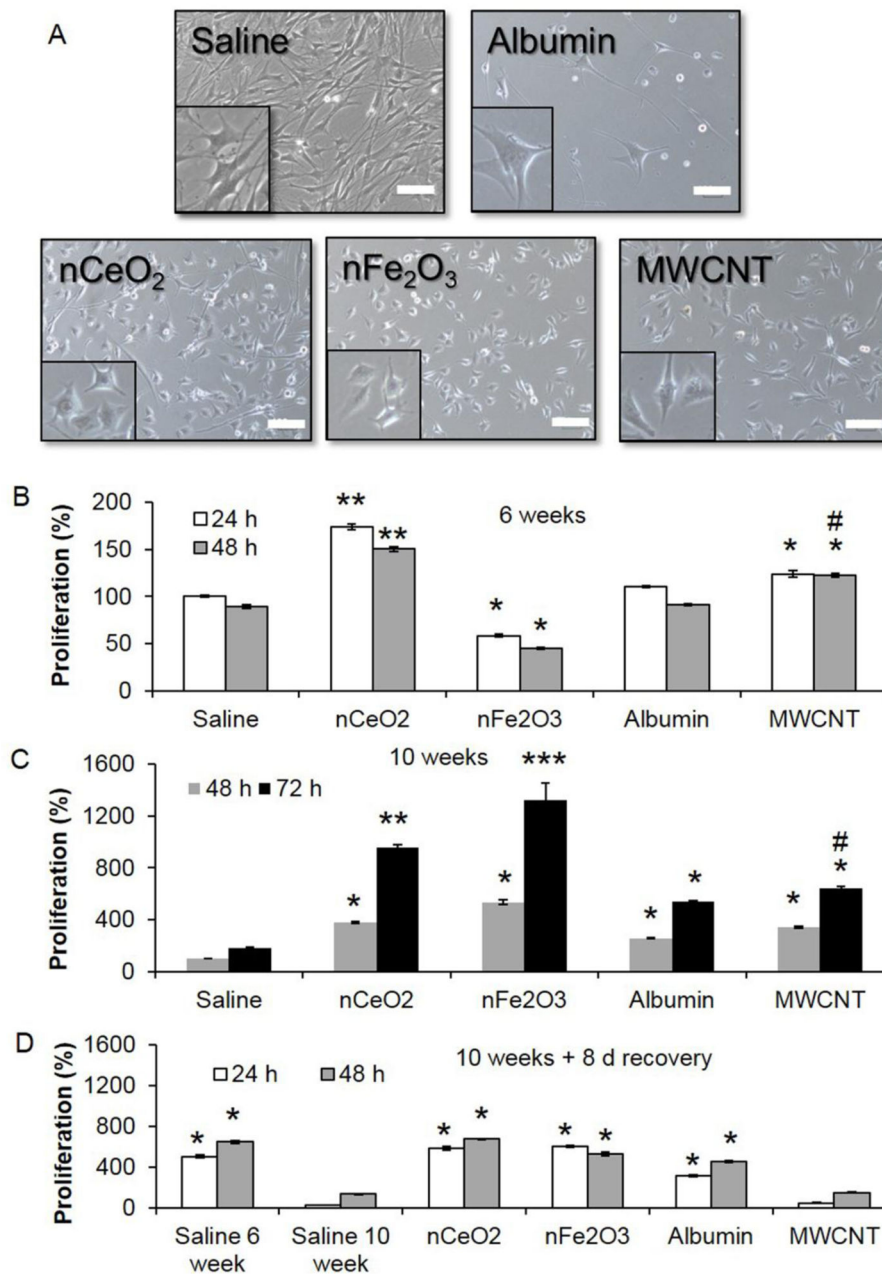
Figure 2. Cell morphology and cell proliferation of nCeO 2 , nFe 2 O 3 , and MWCNT-exposed pSAECs at 6 and 10 weeks after 0.18 μg NMO/cm 2 and 0.06 μg MWCNT/cm 2 exposures. A) At 48 h post-seeding, nCeO 2 , nFe 2 O 3 , and MWCNT exposed cells displayed a more rounded morphology compared to saline passage and low passage pSAECs. Bars and insert width = 200 μm. B) At 6 weeks exposure, nCeO 2 - and MWCNT-exposed cells increased cell proliferation, as measured by WST-1 assay, above respective controls while nFe 2 O 3 -exposed cells experienced a significant reduction. C) At 10 weeks exposure, nFe 2 O 3 -exposed cells possessed the largest significant increase in cell proliferation compared to all treatments. D) Following 8 days recovery in particle-free medium, both nCeO 2 and nFe 2 O 3 retained
