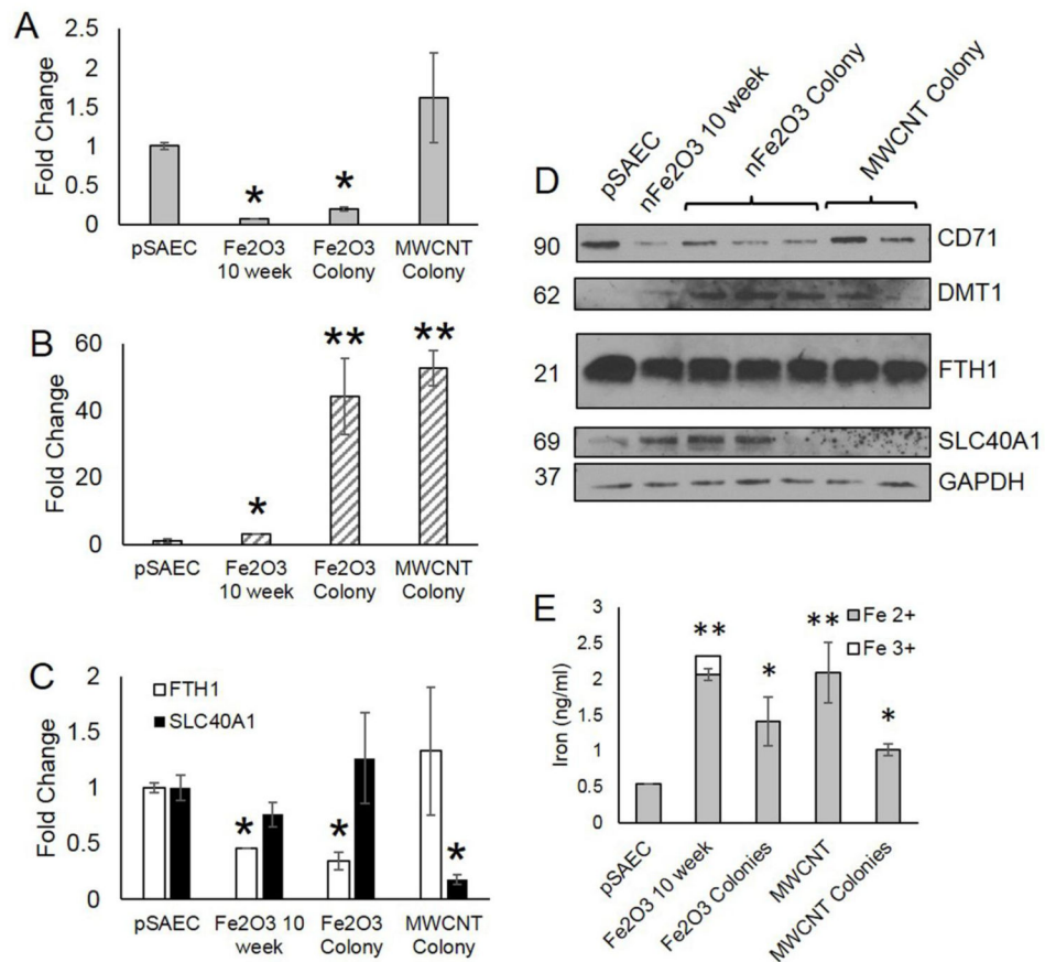
Figure 6. Altered iron homeostasis protein expression and increased intracellular iron levels in nFe 2 O 3 -transformed cells and colony clones. A) Decreased transferrin receptor (CD71) and B) increased divalent metal transporter (DMT1) expression in nFe 2 O 3 -transformed cells and clones compared to low passage, unexposed pSAECs. C) Decreased ferritin (FTH1) expression in nFe 2 O 3 -transformed cells and clones. D) Representative protein bands via SDS-page Western Blot. All densitometry quantification used GAPDH as a loading control. E) Increased intracellular ferrous iron in ENM sub-chronic exposed pSAECs. * indicate a significant difference compared to low passage pSAEC control (p<0.05).
