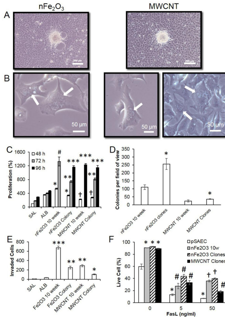
Figure 4. Subclones from 10 week nFe 2 O 3 and MWCNT-exposed pSAEC soft agar colonies retained transformation and several cancer cell hallmark characteristics. A) Plated subclones exhibited foci in confluent plates. B) Multi-nucleated cells were observed in both sub-clone populations. C) Retention of accelerated proliferation compared to 10 week exposure populations, saline-(SAL), and albumin (ALB)-exposed cells, respectively. nFe 2 O 3 10 week absorbance values exceeded detection values at 96 h time point. nFe 2 O 3 - and MWCNT-exposed cells are compared to their respective vehicle control-exposed cells. Different * and # symbols indicate significant differences compared to other treatment groups at each time point. † indicates a significant decrease compared to ALB control (p < 0.05). D) Both nFe 2 O 3 and MWCNT clones exhibited significant increases (*, p < 0.05) in the number of soft agar colonies and E) significant decreases in invasion ability compared to their 10 week transformed counterparts, but above SAL-, and ALB-exposed cells' ability. F) Enhanced apoptosis resistance of nFe 2 O 3 - and MWCNT-exposed cells in the extrinsic pathway compared to low passage pSAECs. Cells were exposed to FasL for 24 h, fluorescently
