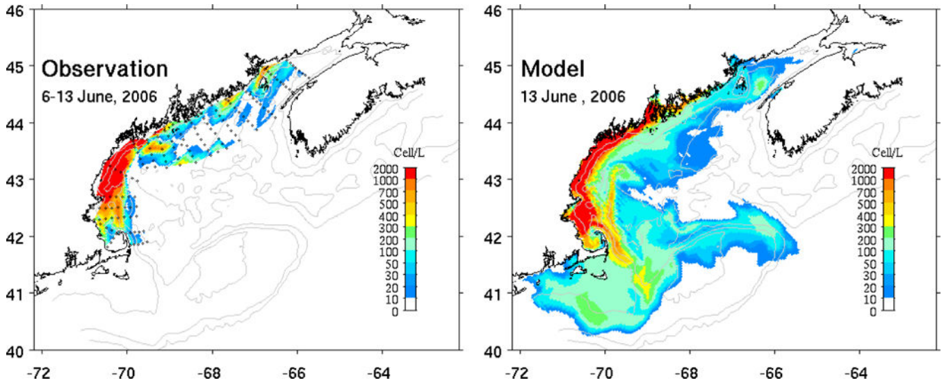
Fig. 7. Comparison of observed (a) and modeled (b) surface Alexandrium fundyense cell concentrations during a bloom in the Gulf of Maine (Li et al. 2009). Open circles denote stations sampled. The model slightly underestimates cell concentrations, but does capture the major features of the extensive coastal bloom.
