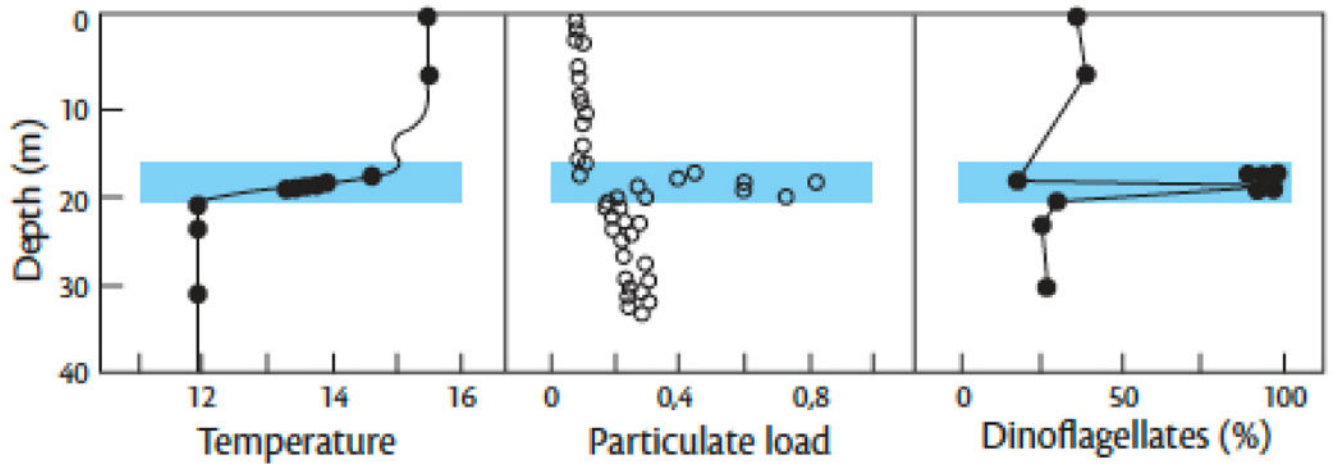
Fig. 5. Vertical distribution of temperature (°C), particulate total volume (relative units), and fractional cell concentration of dinoflagellates (percentage) off the “pertuls d’Antioche,” France. In this example, the HAB species Dinophysis acuminata was a significant component of the dinoflagellate assemblage at the pycnocline, but was absent elsewhere in the water column. (Modified from Gentien et al. (1995).)
