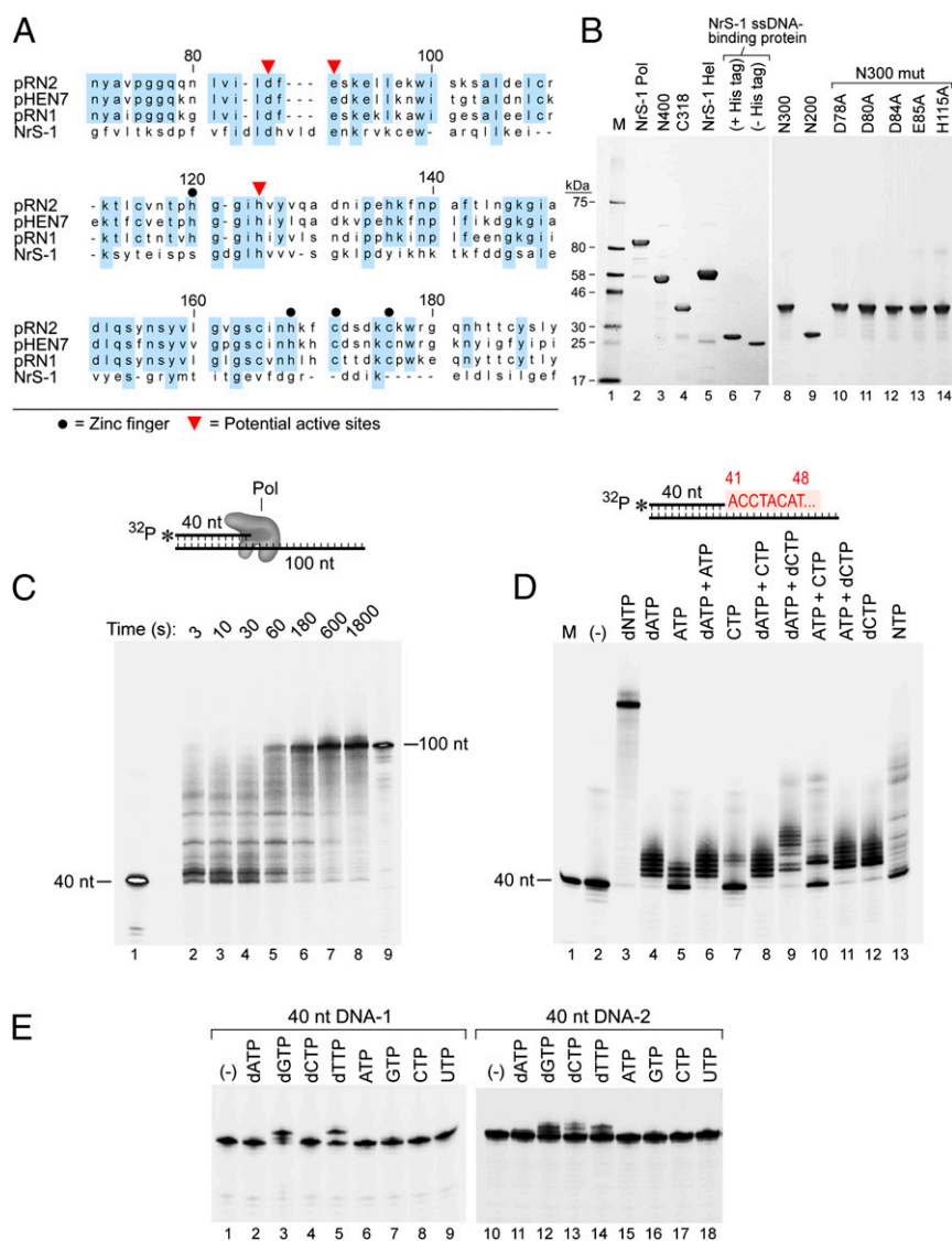
Fig. 1. An unusual DNA polymerase from deep-sea vent phage NrS-1. (A) NrS-1 gene protein 28 shares weak homology to archaeal prim-pols. Alignment between NrS-1 gene protein 28 and three prim-pols encoded by archaeal plasmids (10) was made using CLC Sequence Viewer 6, and the regions containing homology are shown. Identical residues among archaeal prim-pols and those among prim-pols and NrS-1 gene protein 28 are highlighted by blue background. (B) SDS/PAGE gels showing purified proteins analyzed in this work. Lane 1, protein size marker; lane 2, NrS-1 polymerase; lane 3, N-terminal 400 residues of NrS-1 polymerase (N400); lane 4, C-terminal 318 residues of NrS-1 polymerase; lane 5, NrS-1 helicase; lane 6, NrS-1 ssDNA-binding protein; lane 7, NrS-1 ssDNA-binding protein (His-tag removed); lane 8, N-terminal 300 residues of NrS-1 polymerase (N300); lane 9, N-terminal 200 residues of NrS-1 polymerase (N200); lane 10, N300-D78A; lane 11, N300-D80A; lane 12, N300-D84A; lane 13, N300-E85A; lane 14, N300-H115A. All proteins carry an N-terminal His-tag except that in lane 7. (C) Extension of a primer by NrS-1 polymerase. A primed-template (40/100 nt) substrate in which the primer was 5'- 32 P-labeled and was incubated at 100 nM with 200 nM NrS-1 polymerase and 0.5 mM four dNTPs at 50 °C. Aliquots were removed at increasing time and analyzed on a 10% (wt/vol) TBE-urea gel (lanes 2–8). Lanes 1 and 9 contain 5'- 32 P-labeled 40 nt (primer) and the 100 nt complete complement to the template strand, respectively. (D) Nonspecific incorporation by NrS-1 polymerase. A primed-template (40/100 nt) substrate in which the primer was 5'- 32 P-labeled and was incubated at 100 nM with 200 nM NrS-1 polymerase and 0.5 mM of various (d)NTPs at 50 °C for 30 min and then analyzed on a 10% (wt/vol) TBE-urea gel. Lane 1 is the 5'- 32 P-labeled 40 nt marker. Shown in red is the 5' part of the DNA sequence to be synthesized downstream of the primer. (E) 100 nM each of the two 5'- 32 P-labeled 40-nt DNA strand (40 nt DNA-1 sequence 5'-TTTAGGTACCGGTGCCTAGCAGAAGGCCTAATTCTGCAAA-3'; 40 nt DNA-2 sequence 5'-TTTGAGAATTAGGCCTTCTGCTAGGCACCGGTACCTAAA-3') was incubated with 200 nM NrS-1 polymerase and 0.5 mM various (d)NTPs at 50 °C for 30 min and reaction products analyzed on a 10% (wt/vol) TBE-urea gel.
