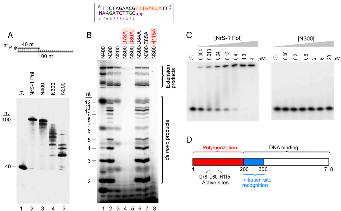
Fig. 4. Active site and functional subdomains of NrS-1 DNA polymerase. (A) Conditions were as in Fig. 1C, except that each reaction was carried out using either 200 nM full-length NrS-1 DNA polymerase (lane 2) or 500 nM of either the N-terminal fragment, N400 (lane 3), N300 (lane 4), or N200 (lane 5). The ability of each of these enzymes to extend 100 nM of a 40/100 nt primed-template was determined. The 40-mer primer is labeled at its 5' end with ^{32}\text{P} . Lane 1 shows the reaction mixture in the absence of enzyme. (B) 10 \mu\text{M} of the 20-nt DNA template containing the NrS-1 polymerase recognition sequence (shown in orange) was incubated with 500 nM of either NrS-1 polymerase fragment N400 (lane 1), N300 (lane 2), N200 (lane 3), or N300 mutants (D78A, lane 4; D80A, lane 5; D84A, lane 6; E85A, lane 7; H115A, lane 8) in the presence of 250 \mu\text{M} each of dATP, dCTP, and dTTP and 25 \mu\text{M} \alpha\text{-}^{32}\text{P} -dGTP at 50 ^{\circ}\text{C} for 30 min. The products were separated on a 25% (wt/vol) TBE-urea gel and analyzed by phosphorimager. Products larger than 20 nt are the result of extension of the templates (Extension Products), whereas those smaller than 13 nt represent abortive and runoff products synthesized de novo ("de novo products"). The runoff product sequence is shown in purple (with the two radioactively labeled G's indicated in green). Numbering of the nucleotides in the product is 5' to 3'. Mutations that abolish NrS-1 polymerase activities are shown in red. (C) In a DNA mobility shift assay, 5 nM of 5'- ^{32}\text{P} -labeled 15 nt DNA (15a) was incubated with the indicated amounts of either full-length NrS-1 polymerase or N300 fragment in the absence of dNTPs for 20 min, followed by loading on a 10% (wt/vol) TBE native acrylamide gel to detect the mobility shift. After electrophoresis, the gel was analyzed using a phosphorimager. (D) A schematic showing the active site and proposed functional subdomains of NrS-1 DNA polymerase.
