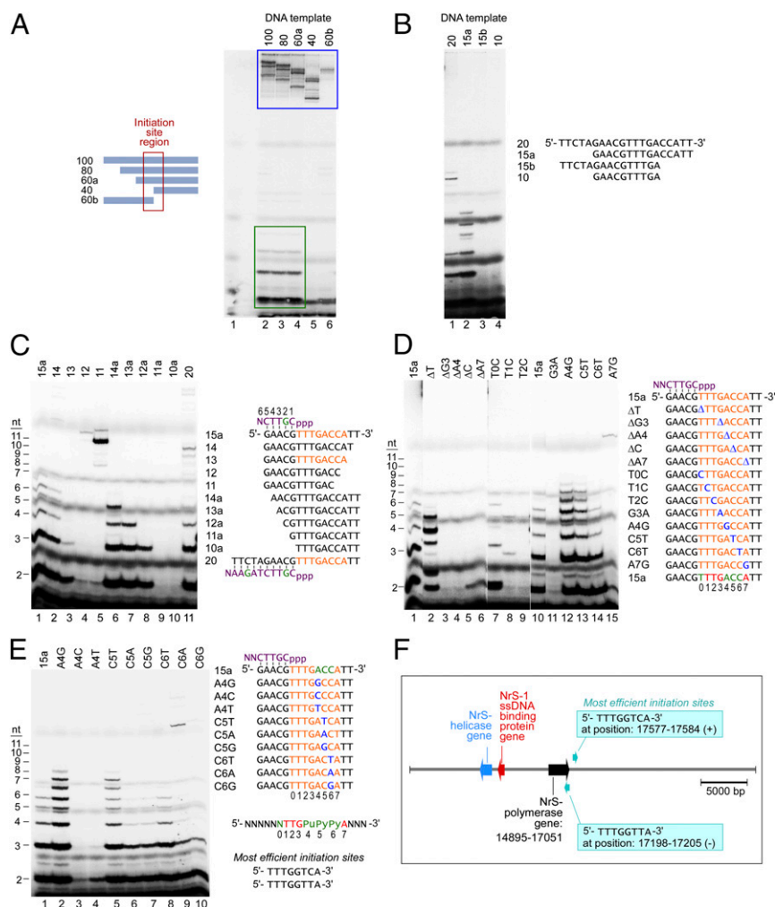
Fig. 3. Nrs-1 DNA polymerase initiates DNA synthesis at specific template sequences. (A) Gel analysis of products synthesized by Nrs-1 DNA polymerase on ssDNA-1 (described in Fig. 2D) and templates that are truncated forms of ssDNA-1. We incubated 10 \mu M 100 nt ssDNA-1 (or its 80, 60, or 40 nt 3' fragments or its 60 nt 5' fragment) with 200 nM Nrs-1 polymerase in the presence of 250 \mu M each of dATP, dCTP, and dTTP and 25 \mu M \alpha - ^{32} P-dGTP at 50 ^{\circ} C for 30 min. The products were separated on a 25% (wt/vol) TBE-urea gel and analyzed by phosphorimager. Extended DNA templates are indicated by the blue box, and the abortive 2–5-nt products are indicated by the green box. The region that contains the potential initiation site is indicated by the red box. (B) We incubated 10 \mu M of either 20-nt, 15-nt, or 10-nt DNA fragments (derived from the sequence within the red box of A) with 200 nM Nrs-1 polymerase in the presence of 250 \mu M each dATP, dCTP, and dTTP and 25 \mu M \alpha - ^{32} P-dGTP at 50 ^{\circ} C for 30 min. And the products were separated on a 25% (wt/vol) TBE-urea gel and analyzed by phosphorimager. (C) DNA templates derived from template 15a in B were tested for whether they could support de novo synthesis by Nrs-1 polymerase. Assay conditions were the same as that described for B. The sequence in orange is the deduced recognition sequence for initiation of de novo synthesis by Nrs-1 polymerase. The sequence of the synthesized product is shown in purple (with the radioactively labeled nucleotide shown in green). Nucleotides in the products are numbered from 5' to 3'. (D) Same assay as that described in C, except that various DNA templates were used that are derived from template 15a, with one nucleotide deletion or replacement (shown in blue) within the recognition region (shown in orange), were tested for their efficiency to support de novo synthesis. Based on these results, the strictly required sequence for template recognition for de novo DNA synthesis is shown at the bottom in red, and those sequences that do not show strict specificity are shown in green. The 8 nt of the recognition sequence are numbered from 5' to 3' as 0–7. (E) Same assay as that described in C, except that various DNA templates were used that are derived from template 15a, with one nucleotide replacement (shown in blue) within the recognition region (shown in orange), were tested for their efficiency to support de novo synthesis. Based on these results, the strictly required sequence for template recognition site for de novo DNA synthesis is shown at the bottom in red, whereas those sequences that are important but do not show strict specificity are shown in green. (F) Position of the Nrs-1 DNA polymerase gene and the two most efficient initiation sites in Nrs-1 genome.
