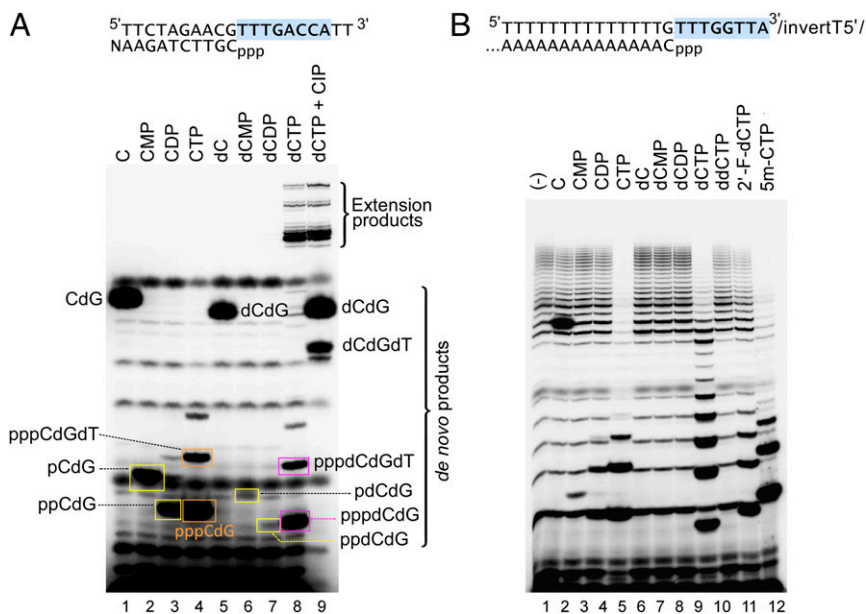
Fig. 5. Nrs-1 DNA polymerase initiates DNA synthesis exclusively with dNTP. (A) The sequence of the 20-nt DNA template used in this experiment is shown at the top, with the Nrs-1 polymerase recognition sequence in blue background and the product sequence shown below the template. We mixed 10 \mu M of this template with 500 nM Nrs-1 DNA polymerase N300 fragment, 250 \mu M dATP, 250 \mu M dTTP, and 50 \mu M \alpha - 32 P-dGTP. The reaction was initiated by the addition of 250 \mu M of either C (lane 1), CMP (lane 2), CDP (lane 3), CTP (lane 4), dC (lane 5), dCMP (lane 6), dCDP (lane 7), or dCTP (lane 8). Reaction mixtures were incubated at 50 °C for 30 min. The products then were separated on a 25% (wt/vol) TBE-urea polyacrylamide gel. The gel was then analyzed using a phosphorimager. Lane 9 contains the same reaction mixture as that in lane 8, except that it was treated with 1 U/ \mu L calf-intestinal alkaline phosphatase at 37 °C for 15 min before loading on the gel. The identities of the major product bands on the gel are annotated. (B) The sequence of the 23-nt DNA template used in this experiment is shown at the top, with the Nrs-1 polymerase recognition sequence in blue background and the product sequence shown below the template. The template was designed for the specificity of Nrs-1 polymerase to produce a product initiated with dCTP and followed by a run of dAMPs (5'-CAAAAAAAAAAAAAA-3'). Reactions were prepared and analyzed as in A above, with the mixtures containing 50 \mu M \alpha - 32 P-dATP and 50 \mu M of either C (lane 2), CMP (lane 3), CDP (lane 4), CTP (lane 5), dC (lane 6), dCMP (lane 7), dCDP (lane 8), dCTP (lane 9), ddCTP (lane 10), 2'-F-dCTP (lane 11), or 5m-CTP (lane 12). Lane 1 contains the control reaction mixture carried out in the absence of any dCTP analogs.
