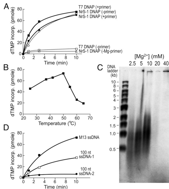
Fig. 2. NrS-1 DNA polymerase synthesizes DNA de novo. (A) 10 nM M13 ssDNA or primed-M13 ssDNA (annealed with M13 primer M2, 5'-CCAG TCAG CAGT-3') was incubated with 100 nM T7 DNA polymerase (solid square, with primer; open square, without primer) or NrS-1 DNA polymerase (solid circle, with primer; open circle, without primer) in the presence of 250 \mu M each of dATP, dGTP, and dCTP and 10 \mu M ^3 H-dTTP; [ Mg^{2+} ] was 5 mM for all assays except that no Mg^{2+} was added for the assay shown by an open triangle, and the incorporation of dTMP into DNA at various time points at 37 °C (for T7 DNA polymerase) or 50 °C (for NrS-1 DNA polymerase) was measured by DE81 (Whatman) filter-binding assay. (B) Effect of temperature on de novo DNA synthesis by NrS-1 DNA polymerase. Reaction conditions were as described for A using 10 nM M13 ssDNA template and 100 nM NrS-1 DNA polymerase. Reactions were carried out for 10 min at the indicated temperatures, and then the incorporation of dTMP into DNA at various time points was measured by DE81 (Whatman) filter-binding assay. (C) De novo DNA synthesis products catalyzed by NrS-1 DNA polymerase on M13 ssDNA were analyzed on 0.8% alkaline agarose gel. Reaction conditions were as described for A, except that nucleotide mixture was 250 \mu M each of dATP, dCTP, and dTTP and 25 \mu M \alpha - ^{32} P-dGTP, and the indicated amounts of MgCl_2 were used. Reactions were carried out for 10 min at 50 °C. (D) De novo DNA synthesis by NrS-1 DNA polymerase on the templates M13 ssDNA (solid square), 100 nt template-1 (open square), and -2 (solid circle) (ssDNA-1 sequence 5'-TAGACTGAATAGTTAAATAGGCAGATATAAAATGGTCAAACGTTCTAGAATATGTAGGTTTTGCAGAATTAGGCCTTCTGCTAGGCACCGGTACCTAAA-3'; ssDNA-2 sequence 5'-TTTAGGTACCGGTGCTAGCAGAAGGCCTAATTCTGCAAACCTACATAGTTCTAGAACGTTTGACCATTTATATCTGCTATTTAACTATTCAGTCTA-3'). Reaction conditions were as described for A, except for the DNA templates used.
