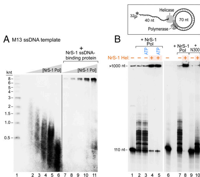
Fig. 6. Coordination between NrS-1 replication proteins. (A) We incubated 10 nM of M13 ssDNA with 250 \mu M of dATP, dCTP, and dTTP and 25 \mu M \alpha - ^{32} P-dGTP in the absence (lanes 2–6) or presence (lanes 7–11) of 30 \mu M NrS-1 ssDNA-binding protein (His-tag removed, as shown in Fig. 1B, lane 7). Reactions were carried out with increasing concentrations of NrS-1 DNA polymerase as follows: 12 nM (lanes 2 and 7), 37 nM (lanes 3 and 8), 111 nM (lanes 4 and 9), 333 nM (lanes 5 and 10), and 1,000 nM (lanes 6 and 11). Reactions were carried out at 50 ^{\circ} C for 30 min. The products were separated on a 0.8% alkaline agarose gel, and then the gel was analyzed by a phosphorimager. Lane 1 contains the 5'- ^{32} P-labeled DNA size marker. (B) DNA synthesis on a minicircle template to measure leading strand DNA synthesis. The primer template consists of a 110 nt 5'- ^{32} P-labeled DNA template annealed to a 70-nt circular template, shown schematically on top of the gel (23). We incubated 50 nM of this template with 200 nM NrS-1 DNA polymerase (lanes 2–5, 7, and 8) and 250 \mu M dNTPs in the absence (lanes 2, 3, and 7) or presence (lanes 4, 5, and 8) of 1 \mu M NrS-1 helicase (shown in Fig. 1B, lane 5). Reaction mixtures were incubated at 50 ^{\circ} C for 30 min. The products were analyzed on a 10% (wt/vol) polyacrylamide TBE-urea gel, and then the gel was analyzed by a phosphorimager. The reaction mixtures in lanes 3 and 5 also contain 1 mM ATP. The reaction mixtures in lanes 9 and 10 contained 500 nM NrS-1 polymerase N300 fragment in place of the full-length NrS-1 polymerase. Lanes 1 and 6 contain the 5'- ^{32} P-labeled 110 nt DNA as a marker for no extension.
