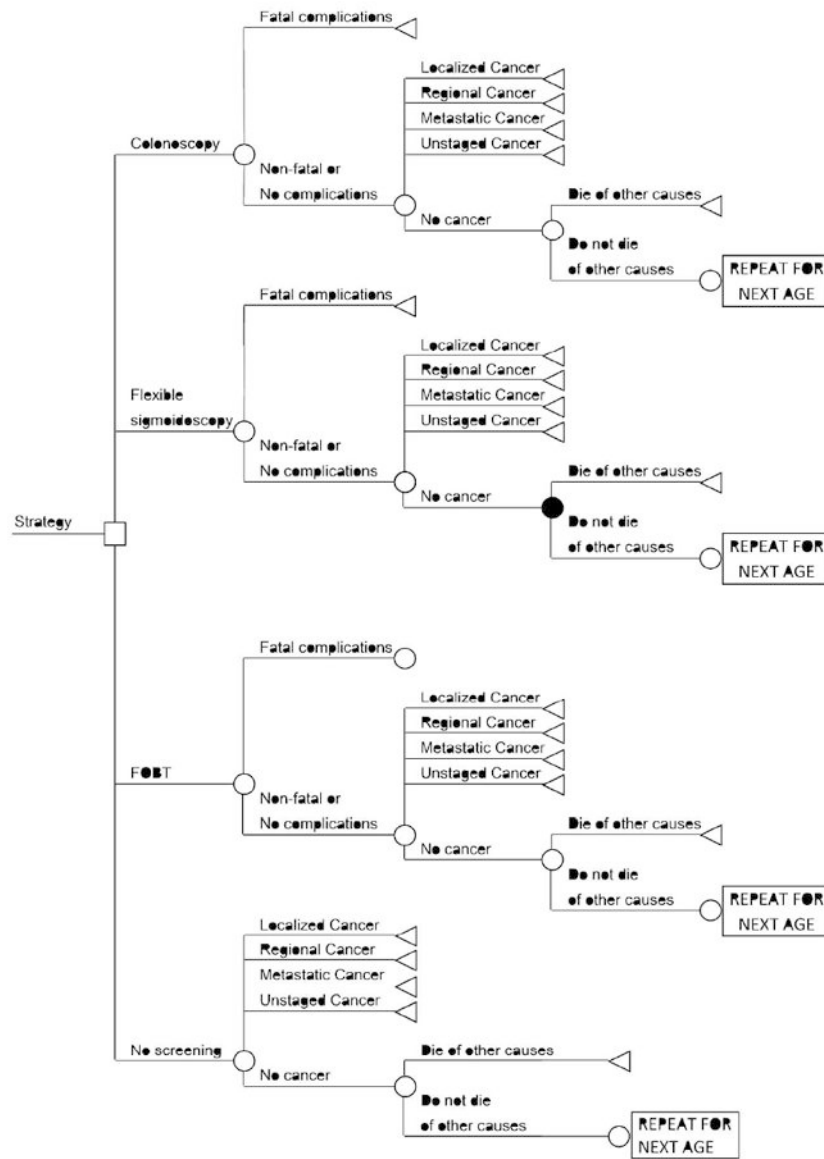
Figure 3. Decision Tree
