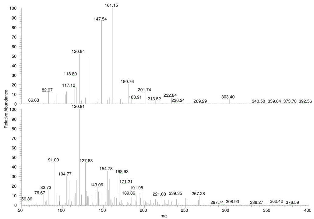
Figure 2. APCI CID mass spectra for cortisol (retention time 12.4 min, bottom panel) and one of its isomer (retention time 11.4 min, top panel).
