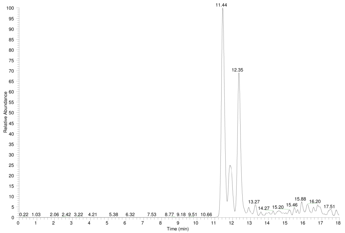
Figure 1. Typical extracted ion chromatograph of cortisol and its isomers in human eccrine sweat (363→121 transition).
