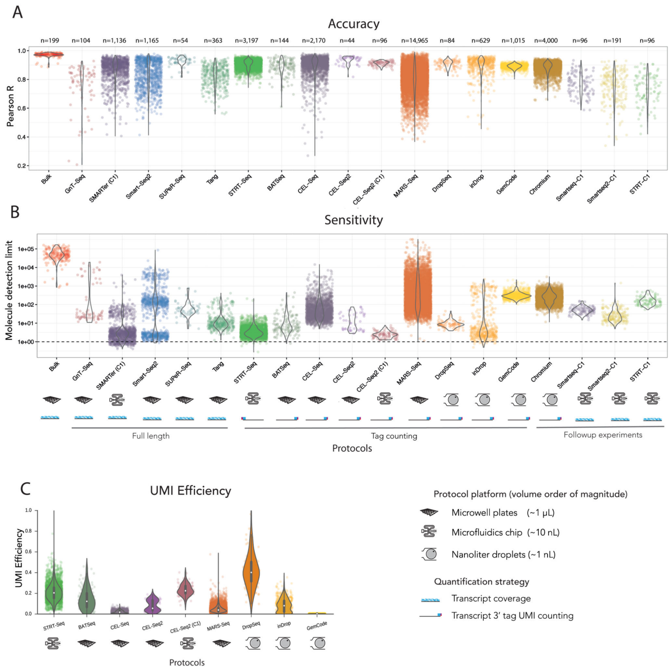
Figure 2. Comparison of performance metrics for different protocols. (A) Accuracy. Distributions of Pearson correlations ( R ) of all samples stratified by protocol investigated (without accounting for sequencing depth). (B) Sensitivity. Distributions of molecule detection limits of all samples stratified by protocol (without accounting for sequencing depth). The number of samples ( n ) is highlighted above the protocols. The implementation platforms and quantification strategies are indicated below the protocols. (C) UMI Efficiency. Distributions of UMI counting efficiencies in UMI-tag counting based samples, stratified by protocols. For the analysed UMI based data, the UMI efficiency recapitulates the logistic regression based molecule detection limit.
