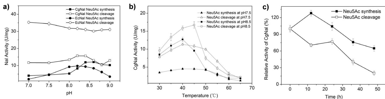
Figure 3 | Effects of pH and temperature on CgNal activity. (a) Effects of pH on CgNal and EcNal, (b) Effects of temperature on CgNal at pH7.5 and pH8.5, (c) CgNal stability at pH 8.5, 40°C.
