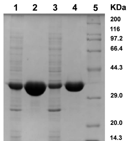
Figure 2 | SDS-PAGE analysis of CgNal and EcNal. Lane 1, supernatant of pET28a-CgNal-Rosetta cell lysate, Lane 2, purified CgNal, Lane 3, supernatant of pET28a-EcNal-Rosetta cell lysate, Lane 4, purified EcNal. CgNal and EcNal were cultivated, induced, purified and sampled under the same conditions.
