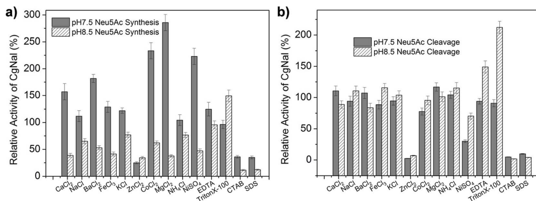
Figure 4 | Effects of salts and detergents on CgNal activity. (a) Effects of salts and detergents to CgNal activity on Neu5Ac synthesis at pH7.5 and pH8.5 (b) Effects of salts and detergents to CgNal activity on Neu5Ac cleavage at pH7.5 and pH8.5.
