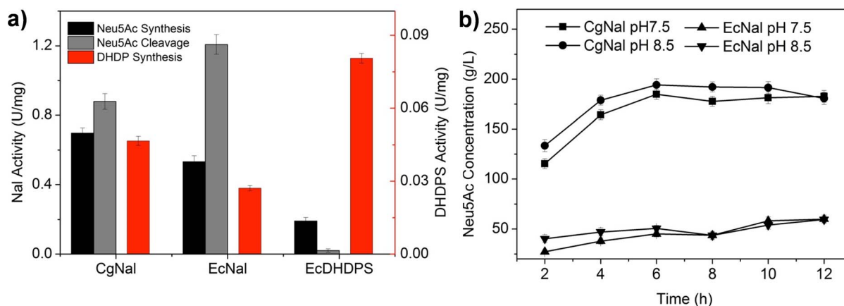
Figure 6 | (a) Comparison of enzyme activity with different substrate of CgNal, EcNal and EcDHDPS. (b) Synthesis of Neu5Ac by CgNal and EcNal. In a reaction mixture containing 0.8 M ManNAc, 2 M pyruvate and 0.5 M Tris-HCl (pH 7.5 and pH 8.5) purified EcNal or CgNal was added to initiate the synthesis.
