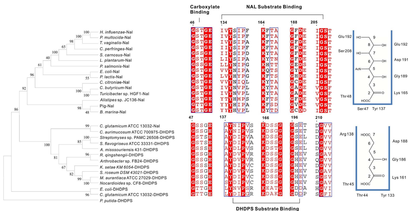
Figure 5 | Phylogenetic tree of CgNal and alignment of key residues. The phylogenetic tree was constructed and visualized with MEGA 5.2 39 . BLAST identified DHDPS and NAL homologous to CgNal to construct the phylogenetic tree, Pseudomonas putida KDGDH (GenBank accession: P42233.1) was defined as the outgroup. The details of alignment outputs are shown in the middle of the figure. The schematic diagram showing modulation of residues within the active site of NAL and DHDPS is shown on the right side of the figure.
