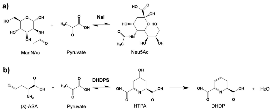
Figure 1 | Reactions catalyzed by (a) Nal and (b) DHDPS.
