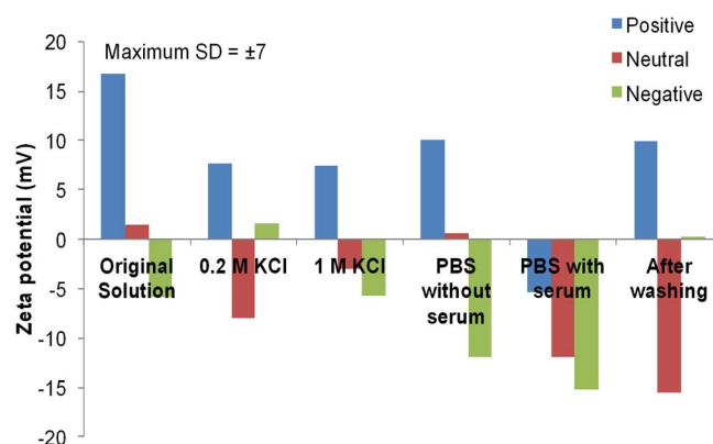
Figure 2 | Zeta potential measurements of different surface-charged PVA-coated SPIONs in water (original solution), 0.2 M KCl, 1.0 M KCl, PBS without serum, PBS with serum and NPs after 30 column-volume washings with PBS.
