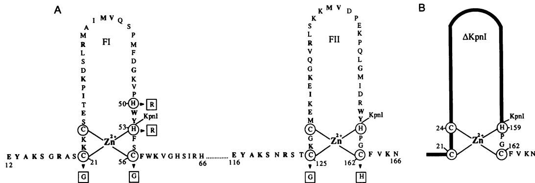
FIG. 2. Structure of the zinc-binding domain and mutagenesis. (A) The zinc-binding domain is drawn to show two zinc-coordinated fingers. Finger I (FI) is shown using Cys-21, Cys-24, His-53, and Cys-56 to coordinate Zn(II), and finger II (FII) is shown using Cys-125, Cys-128, His-159, and Cys-162 to coordinate Zn(II). Duplicated amino acids are shown in boldface according to refs. 6 and 7. Amino acid substitutions are indicated by arrowheads pointing to the mutant amino acids. Locations of Kpn I sites are shown next to the sequence. The mutants are described in Table 1. (B) Putative hybrid zinc finger (FI/FII) of \Delta KpnI deletion mutant. Heavy line represents FI sequence.
