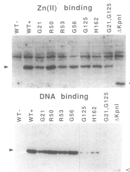
FIG. 4. Zinc and DNA binding activity. Wild-type [WT, noninduced (-) or induced (+)] and mutant PARP fusion polypeptides in crude E. coli extracts were subjected to SDS/12% PAGE, transferred to nitrocellulose, and probed either with ^{65}\text{Zn(II)} (Upper) or with a ^{32}\text{P} -end-labeled DNA probe harboring a single-strand break (Lower). The blots were autoradiographed. Arrowheads mark the position of the fusion proteins.
