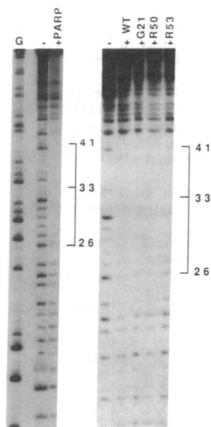
FIG. 5. DNase I footprint assays for the protection of a single-strand break in DNA by the PARP zinc-finger domain expressed in E. coli . Wild-type (WT) and mutant PARP polypeptides in crude E. coli lysates were subjected to SDS/12% PAGE, transferred to nitrocellulose, and incubated with a 32 P-end-labeled double-stranded DNA probe (66 bp) harboring a single-strand break at position 33 (16). DNase I footprint assays were performed as described under Materials and Methods . (Left) Lane G, degradation products of the guanine-specific sequencing reaction; lane -, control for DNA degradation without PARP; lane +PARP, footprint of purified calf thymus PARP. (Right) Lane 1, control for DNA degradation without PARP; lane +WT, footprint of PARP wild-type zinc-finger domain; lanes +G21, +R50, and +R53; footprints of G21, R50, and R53 mutants. Protected region extending 7 nucleotides on either side of position 33 is bracketed.
