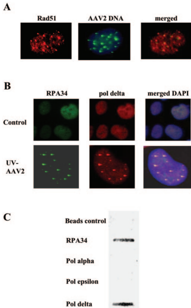
FIG. 4. UV-AAV2 DNA colocalizes with damage-responsive proteins and with DNA polymerase delta, which binds UV-AAV2 DNA directly. (A) For combined protein immunofluorescence and in situ hybridization for the viral DNA, cells were plated onto gridded coverslips and infected with UV-AAV2 as described in the legend of Fig. 3. Cells were processed 2 days postinfection as described in Materials and Methods. Rad51 protein foci, representing the proteins that form foci after UV-AAV2 infection, colocalized with UV-AAV2 DNA foci. (B) U2OS cells were plated onto coverslips and infected as described above. Two days postinfection, cells were processed for detection of immunofluorescence with antibodies against RPA and DNA polymerase (pol) delta and chromatin staining with DAPI. UV-AAV2 infection caused polymerase delta to accumulate into nuclear foci, which colocalized with RPA foci. Controls show RPA- and polymerase delta-specific staining in noninfected cells. (C) U2OS cells were infected with UV-AAV2 at an MOI of 5,000. Two days postinfection, cells were processed for chromatin immunoprecipitation as described in Materials and Methods. UV-AAV2 was immunoprecipitated without antibodies (beads control) or with antibodies against RPA (RPA34), polymerase alpha, polymerase epsilon, or polymerase delta. DNA from immunoprecipitates was slot blotted and probed with AAV2-specific probes. RPA and polymerase delta bind directly to UV-AAV2 DNA.
