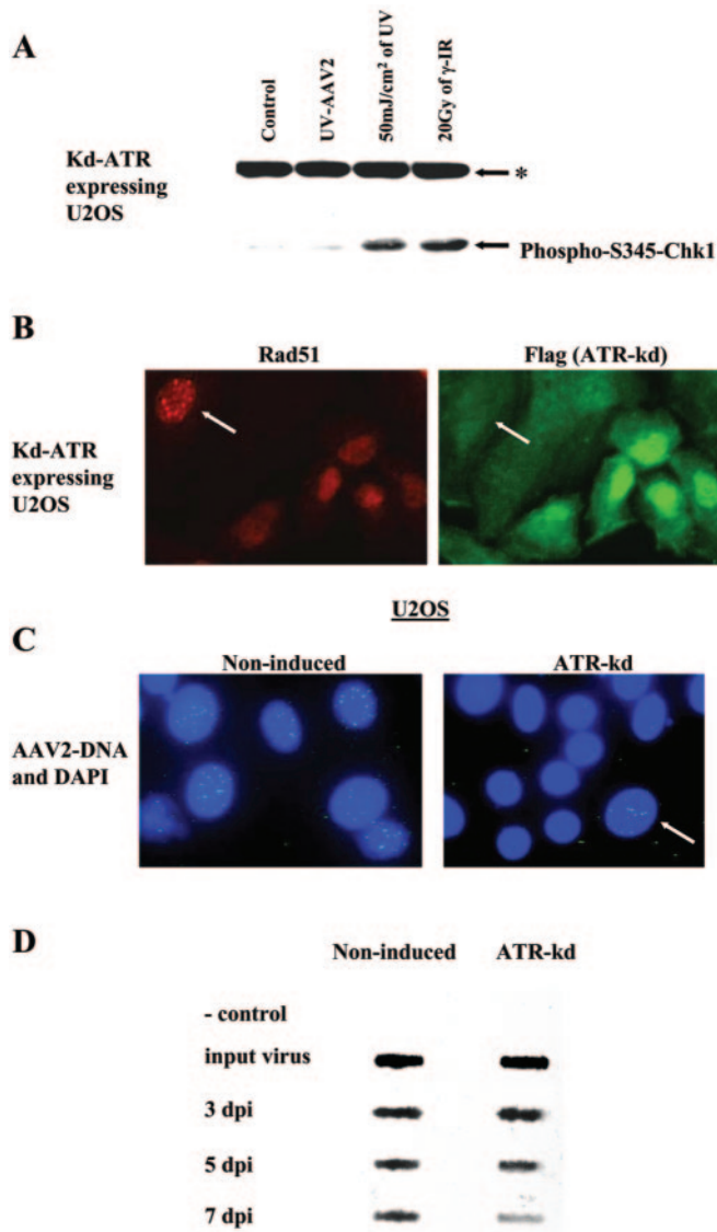
FIG. 6. Expression of kinase-dead ATR abolishes Chk1 phosphorylation, prevents the formation of protein and UV-AAV2 DNA nuclear foci, and exposes UV-AAV2 DNA to nucleases. (A) U2OS cells inducible for kd-ATR were doxycycline induced 1 day before infection with UV-AAV at an MOI of 10,000, and proteins were collected 1 day postinfection (UV-AAV2). Controls include noninfected cells (Control) and cells treated with 50 mJ of UV irradiation/cm 2 and 20 Gy of gamma irradiation ( \gamma -IR). * denotes an unspecific band. (B) kd-ATR-expressing cells were infected with UV-AAV2 as described above and stained for immunofluorescence against Rad51 and Flag. The kd-ATR protein has a Flag tag which enables cells which were successfully induced for kd-ATR expression to be distinguished. The white arrows point out a cell that does not express Flag-tagged kd-ATR and where Rad51 still does form nuclear foci. (C) For in situ hybridization against UV-AAV2 DNA, cells were infected with UV-AAV2 and processed as described in Materials and Methods 2 days postinfection. UV-AAV2 DNA forms nuclear foci in U2OS cells but not in cells induced to express kd-ATR. The white arrow indicates an internal control cell which probably failed to express kd-ATR as judged by its cell cycle-arrested appearance (enlarged nucleus). (D) U2OS noninduced cells and cells induced to express kd-ATR were infected with UV-AAV2 at an MOI of 5,000 and were collected 3, 5, and 7 days postinfection (dpi). DNA was isolated from all the cells on a plate, and the whole yield of DNA was slot blotted and hybridized with an AAV2-specific
