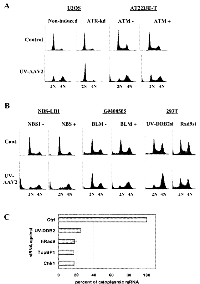
FIG. 2. UV-AAV2 infection-induced G 2 arrest is dependent on ATR, BLM, and Rad9, but not on ATM or NBS1, proteins. (A) U2OS cells not induced or doxycycline induced to express kinase-dead ATR and ATM-deficient and ATM-complemented human fibroblast cells (AT221JE-T) were infected with UV-AAV2 at an MOI of 5,000, and the cellular DNA profiles were determined by FACS analysis 3 days postinfection. For all the FACS analyses in this work, DNA profiles are shown for infected (UV-AAV2) and noninfected (Control) cells, and cellular DNA content is indicated by 2N and 4N. (B) Human transformed fibroblasts (NBS1-LB1) deficient for NBS1 protein and the complemented derivative cells were infected with UV-AAV2 at an MOI of 5,000 and collected for DNA FACS analysis 3 days after infection. The transformed human fibroblast cell line GM08505, which contains inactive BLM protein and the BLM-complemented derivative, were infected at an MOI of 50,000, and cells were collected for DNA FACS analysis 3 days postinfection. 293T cells expressing siRNAs against UV-DDB2 and Rad9 proteins were selected for 3 days, after which they were infected with UV-AAV2 at an MOI of 1,000 and collected 1 day postinfection for FACS. (C) Cells were selected for 3 days for siRNA expression, after which cytoplasmic mRNA was collected and reverse transcribed, and the produced cDNA was analyzed with real-time LightCycler PCR. Error bars are given for triplicates of one RT-PCR experiment. siRNA expression reduced the mRNA levels of UV-DDB2 by 75%, Rad9 by 82%, TopBP1 by 83%, and Chk1 by 89%. The cellular effects of siRNA expression against TopBP1 and Chk1 are shown in Fig. 5B.
