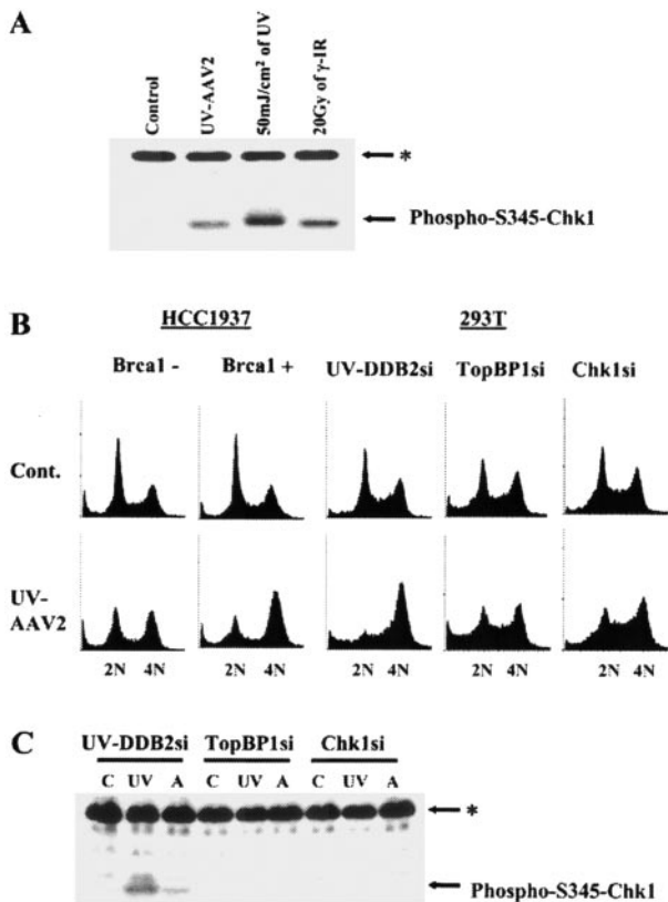
FIG. 5. Phosphorylation of Chk1 protein is needed for proper establishment of G_2 arrest after UV-AAV2 infection. (A) U2OS cells were infected with UV-AAV2 as described in the legend of Fig. 3, and proteins were collected for phospho-S345-Chk1 Western blot 1 day postinfection (UV-AAV2). For controls, proteins were collected from nontreated U2OS cells (Control) and cells treated with 50 mJ of UV irradiation/cm 2 and 20 Gy of gamma irradiation ( \gamma -IR) 4 h after respective treatments. * denotes an unspecific band. (B) The breast carcinoma cell line HCC1937 expressing truncated Brcal and the functional Brcal-complemented cell line were infected with UV-AAV2 at an MOI of 5,000 and collected for FACS analysis 3 days postinfection. 293T cells expressing siRNAs against UV-DDB2, TopBP1, and Chk1 proteins were selected for 3 days, after which they were infected with UV-AAV2 at an MOI of 1,000 and collected 1 day postinfection for FACS analysis. Cont., control. (C) Cells expressing siRNAs against UV-DDB2, TopBP1, and Chk1 were either untreated (C), UV irradiated with 20 mJ/cm 2 (UV), or infected with 1,000 MOI of UV-AAV2 (A), and proteins were collected for Western blot and probed with phospho-S345-Chk1 antibody. * denotes an unspecific band.
