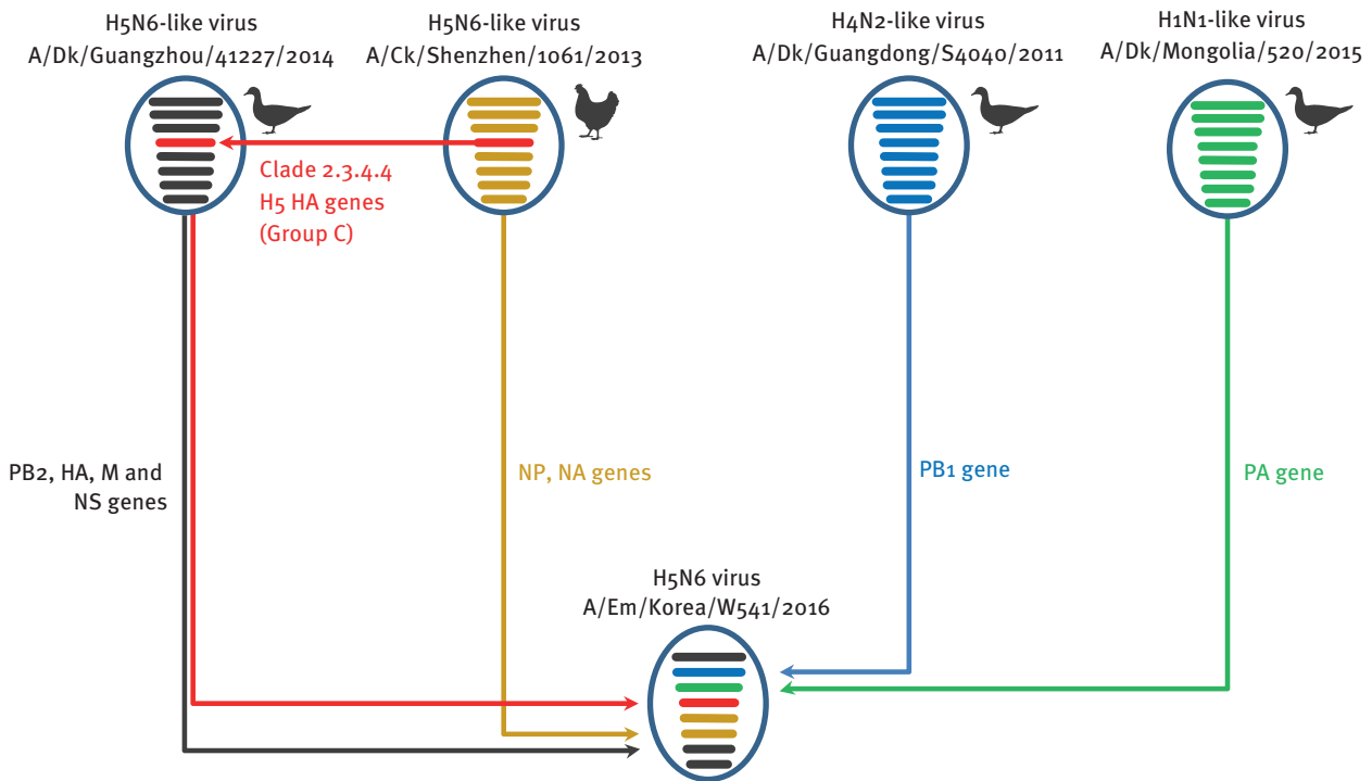
Illustration of genotypes and reassortment events resulting in the novel avian influenza H5N6 virus isolated in South Korea, November 2016
