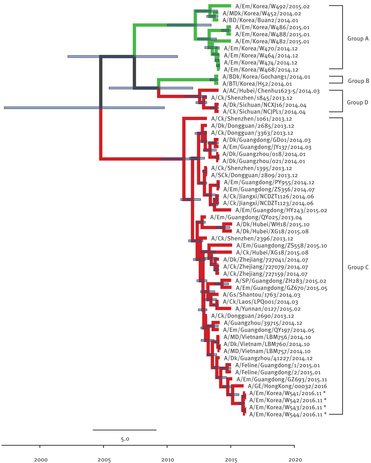
Phylogenetic tree of H5 segment of novel H5N6 viruses, South Korea, November 2016
