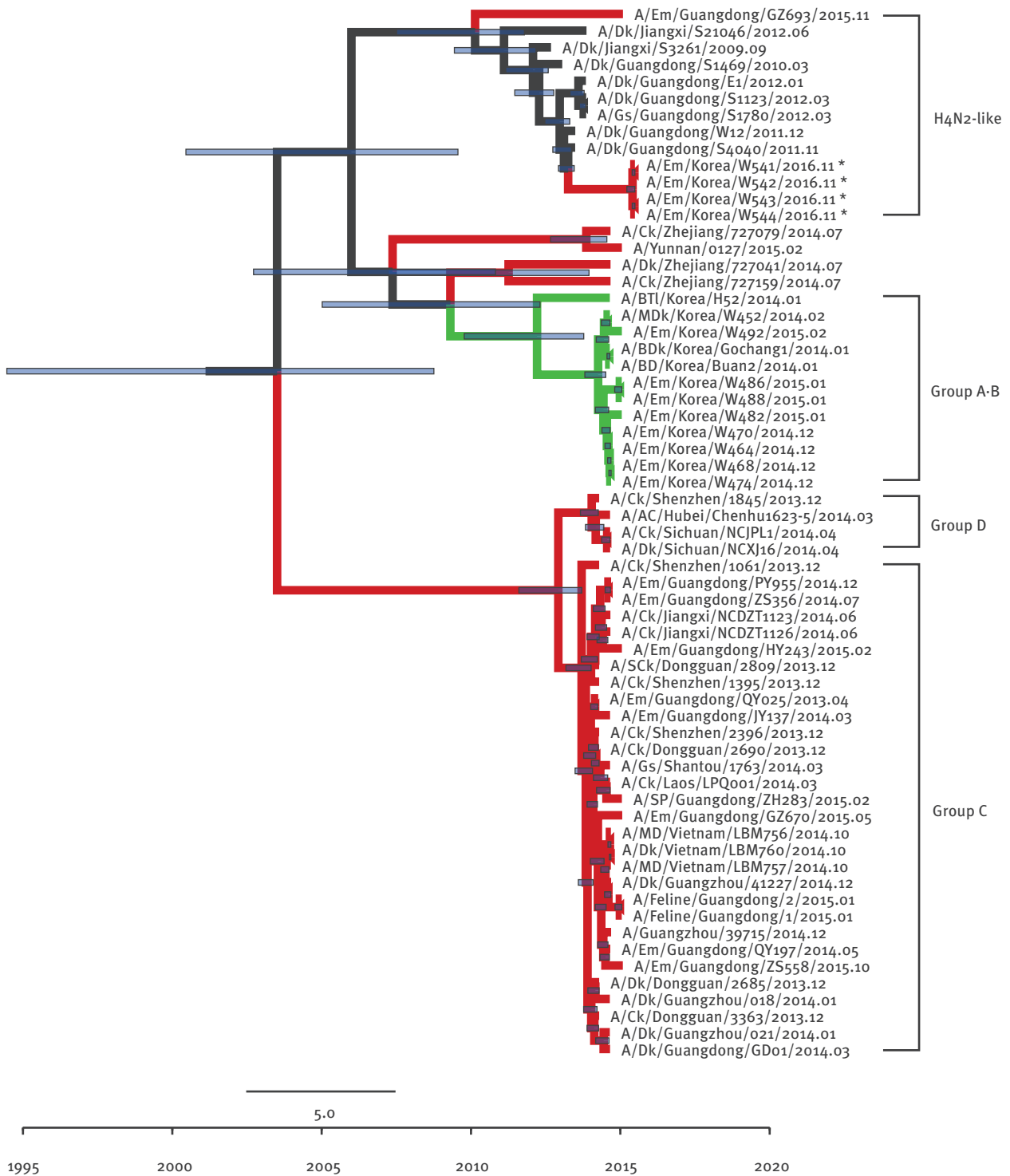
Phylogenetic tree of PB1 segment of novel H5N6 viruses, South Korea November 2016
