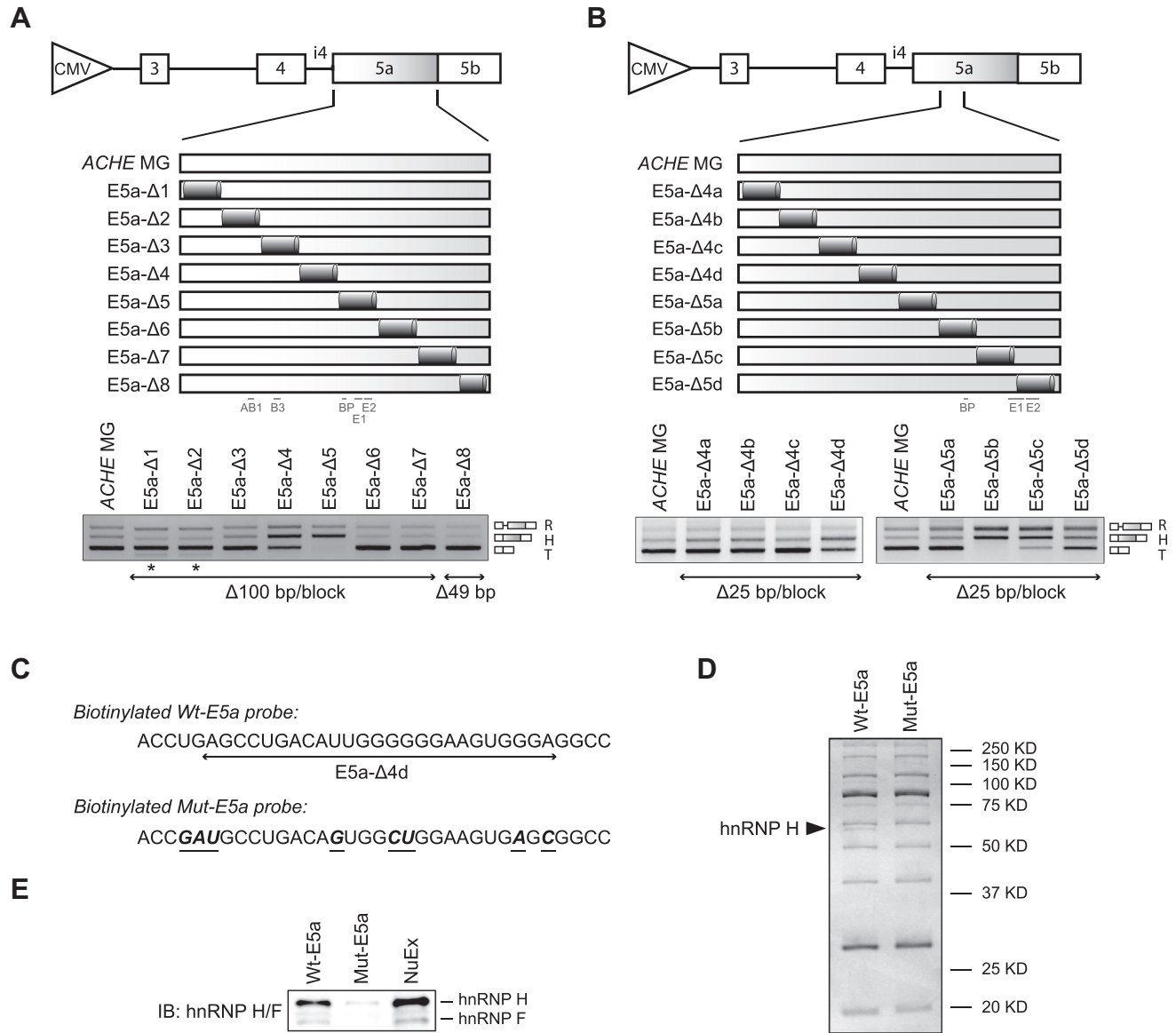
Figure 2. Identification of splicing regulatory cis -elements and trans -acting factors. (A and B) Structure of the human ACHE minigene (MG) construct spanning exons 3 to 5b, which is driven by a CMV promoter. Schematic of scanning deletion mutagenesis of (A) 100-bp and 49-bp blocks of the entire exon 5a and (B) 25-bp blocks of E5a-Δ4 and E5a-Δ5. RT-PCR of the wild-type and deletion constructs transfected in SH-SY5Y cells are shown. ACHE isoforms are schematically shown on the right side of the gel images. Asterisks indicate that the reverse primer for detecting AChE R and AChE H are different from the others, because the primer-binding site is deleted in these constructs. Previously identified regulatory cis -elements (AB1, B3, E1, E2 and the branch point (BP)) (14) in rat Ache are aligned to human ACHE , and are indicated below the schemes. Note that BP is more conserved than the other 4 elements (see Supplementary Figure S2A). (C) Sequence of biotinylated wild-type (Wt) and mutant (Mut) E5a probes covering the E5a-Δ4d region. Mutations are shown in bold italic characters with underlines. (D) Coomassie blue staining of the RNA affinity-purified proteins of SH-SY5Y nuclear extract using the indicated biotinylated RNA probes. Protein size markers are indicated. Mass spectrometry analysis revealed that a distinct protein band of ~55 kDa (arrowhead) is hnRNP H. (E) Immunoblotting of the RNA affinity-purified proteins in (D) with an antibody recognizing both hnRNP H and F.
