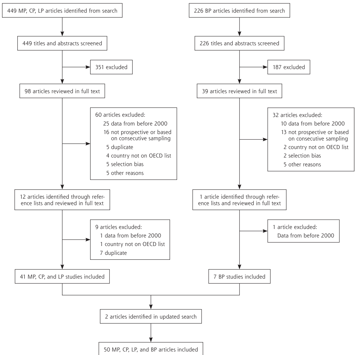
Figure 1. PRISMA diagram.
