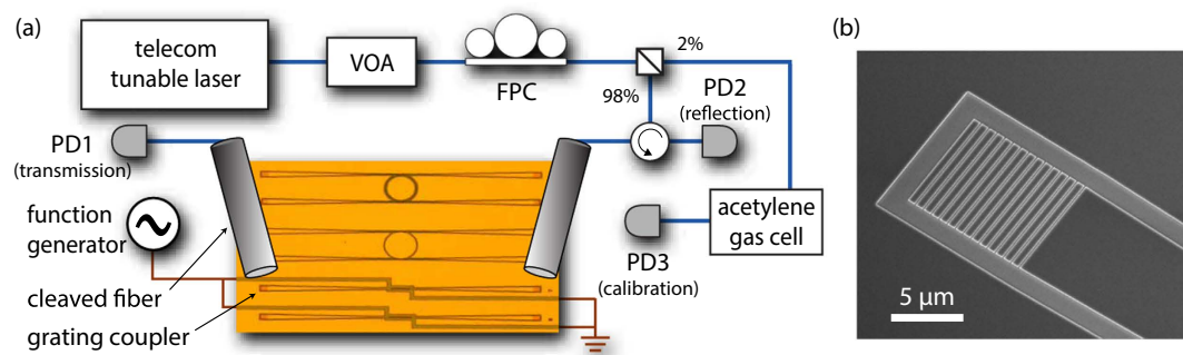
Figure 2. Experimental setup. (a) Diagram of the experimental setup for making optical transmission measurements. (b) Scanning electron micrograph of a typical SiLN grating coupler used in these experiments.
