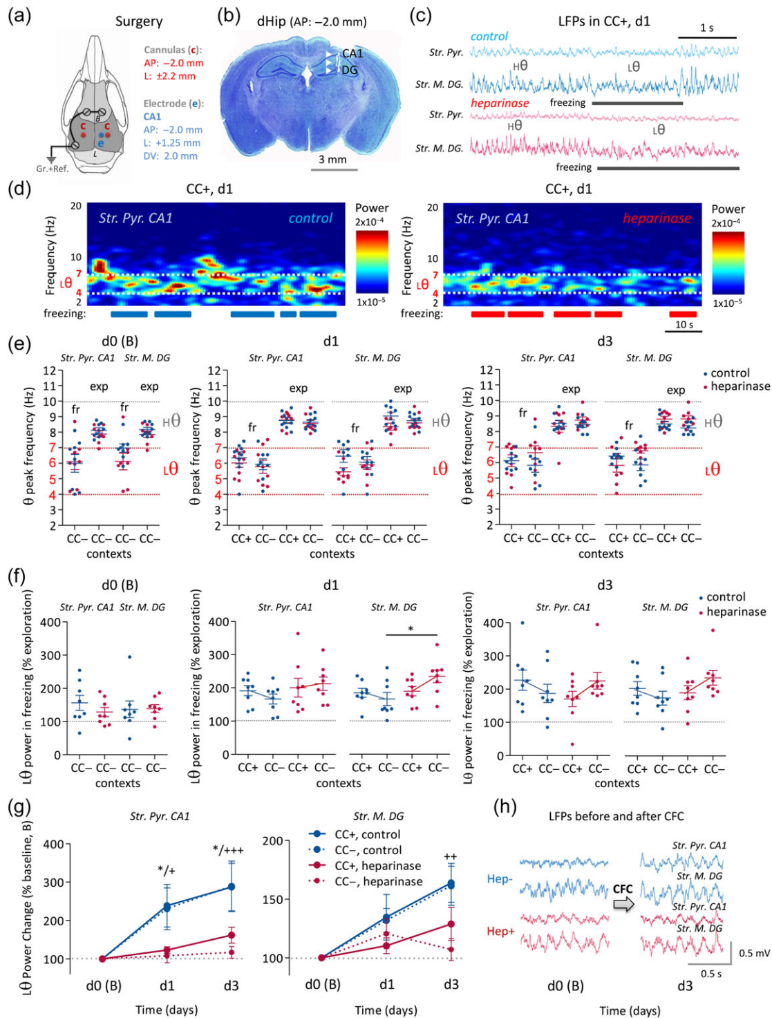
Figure 7. Theta oscillations during CFC are modified by intrahippocampal heparinase injection. (a) Schematic of surgical implantation of hippocampal electrodes and cannulas into a mouse brain with given coordinates and specific arrangement for a HIME system (Senkov et al. 2015). (b) Nissl staining of a brain section with located electrode tracks at the right dorsal hippocampus depicting the tips of the deepest electrodes at the DG and the most superficial electrodes at pyramidal cell layer of CA1. (c) Representative epochs of LFPs in both recorded areas (CA1 and DG) and in both treatment groups showing high theta oscillations (H \theta : 7–10 Hz) while mice explore the conditioned context (CC+) and low theta (L \theta : 4–7 Hz) when they freeze. (d) Representative examples of spectrograms of low frequency oscillations (2–20 Hz) in CC+ for 5 min at d1 after heparinase or control injection. Low theta oscillations show high power specifically at freezing events, while high theta appears only during exploration/motion epochs. Heparinase-injected mice show a reduction in power of low theta oscillations during retrieval of CFC memory traces versus control. (e) Analysis of \theta peak frequency over all recording days shows a \theta frequency shift from H \theta (7–10 Hz) to L \theta (4–7 Hz) of both treatment groups when mice explore (exp) either context (CC+/CC-) and freeze (fr). (f) Analysis of relative L \theta power during freezing normalized over L \theta power during exploration behavior shows a distinct increase (~100%) of L \theta power during freezing in CC+ and a lower increase in CC- in control mice. In heparinase-injected animals, a qualitatively opposite effect was detected, that is L \theta power increased in CC- during freezing more than in CC+. (g, h) The averaged low (4–7 Hz) theta power after CFC was normalized to the prefree conditioning level (baseline, B). A prominent increase of L \theta power can be detected after CFC in control experiments but not in heparinase-injected animals (sample traces in h; * significant difference of theta power in CC+ contexts between 2 treatment groups; +, ++, +++ significant difference of theta power in CC- contexts between 2 treatment groups).
