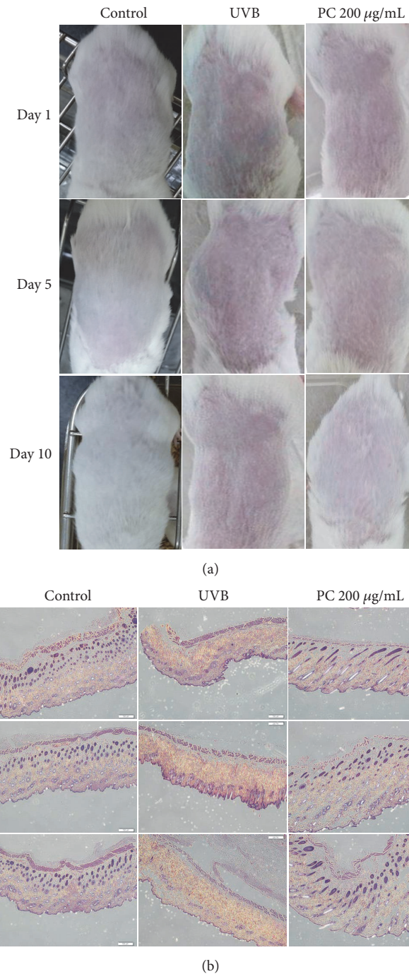
FIGURE 5: Effect of topical treatment of mouse skin with P. cicadae on UVB-induced damage. (a) ICR mice skin was treated with either 200 µg/mL P. cicadae or PBS and was exposed to UVB every 5 days, as described in Methods. Mouse skin treated topically with P. cicadae before UVB exposure reduced UVB-induced signs of sunburn tissue damage. (b) Skin biopsies were processed by H&E staining by a routine procedure. Micrographs show representative findings of skin in response to UVB, sampled after UVB exposure, and a representative section of H&E staining from three independent experiments is shown. Pretreatment of P. cicadae inhibited UVB-induced extensive structural damage in both epidermis and dermis (magnification, 40x).
