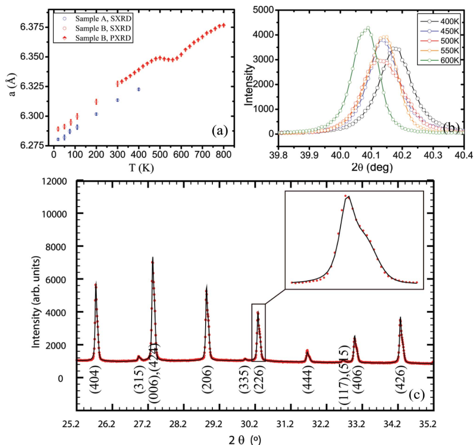
Figure 3 (a) The cell parameters of samples A and B from synchrotron single-crystal X-ray diffraction (SXR) and conventional powder X-ray diffraction (PXR). (b) The (204) reflection plotted as a function of temperature collected with a conventional X-ray source (sample B ). (c) A high-resolution synchrotron PXR pattern showing asymmetries at 550 K (sample B ).
