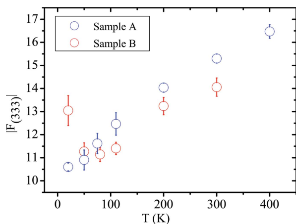
Figure 9 The temperature dependence of F_{333} on an absolute scale for samples A and B from single-crystal diffraction data.
