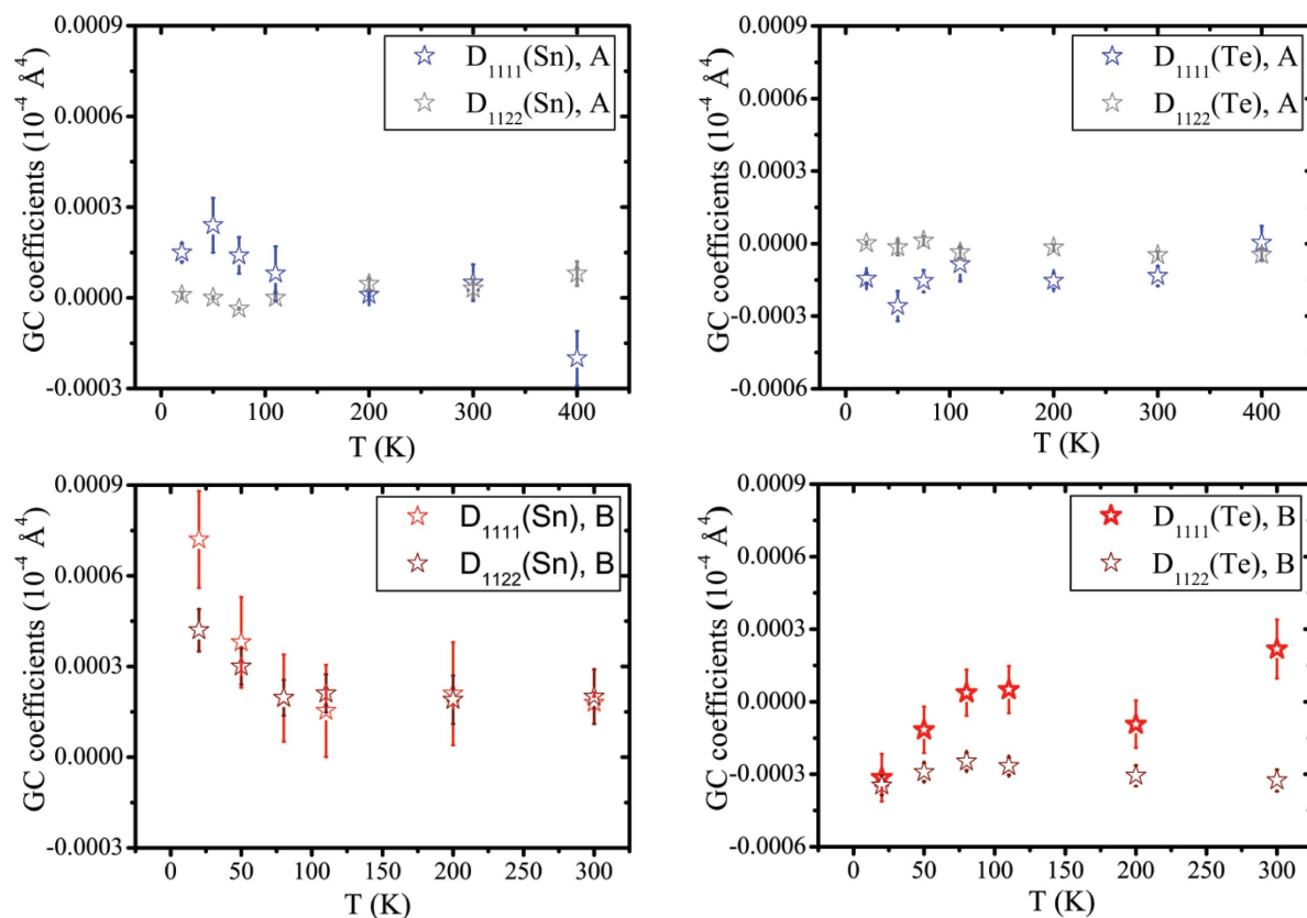
Figure 5 Gram–Charlier parameters of samples A and B when only one atom is refined anharmonically while the other is kept harmonic.
