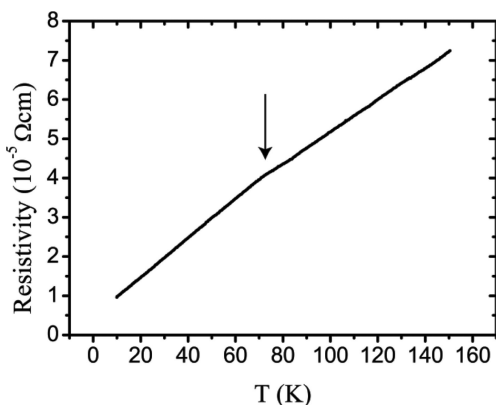
Figure 1 The measured resistivity of sample B using the PPMS. The arrow marks a kink in the resistivity. A similar kink was interpreted as evidence of a structural phase transition by Kobayashi et al. (1976).
