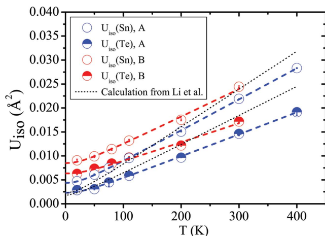
Figure 4 The ADPs of Sn and Te for samples A and B from synchrotron SXR in comparison with the theoretical values from Li, Ma et al. (2014). The coloured dashed lines represent fits to a Debye model.
