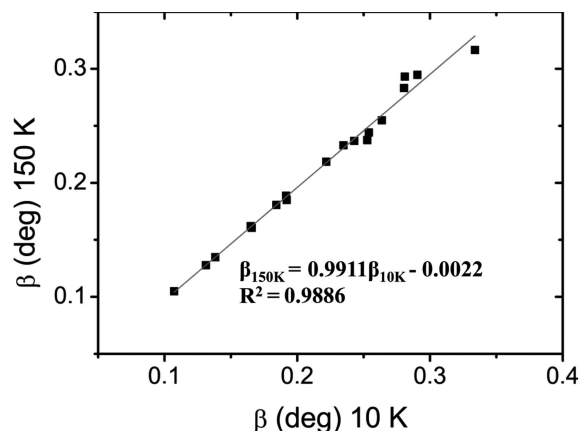
Figure 11 The integral breadth at 150 K versus that at 10 K for reflections in the range 12.9 < 2\theta < 46.8^\circ [ \lambda = 0.50036 (7) Å] with no peak overlap, and that are supposed to split in a transition Fm\bar{3}m \rightarrow R3m .
