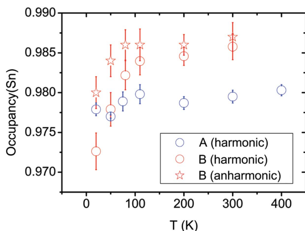
Figure 6 The Sn occupancy in samples A and B from synchrotron SCXRD when only Sn is refined anharmonically.
