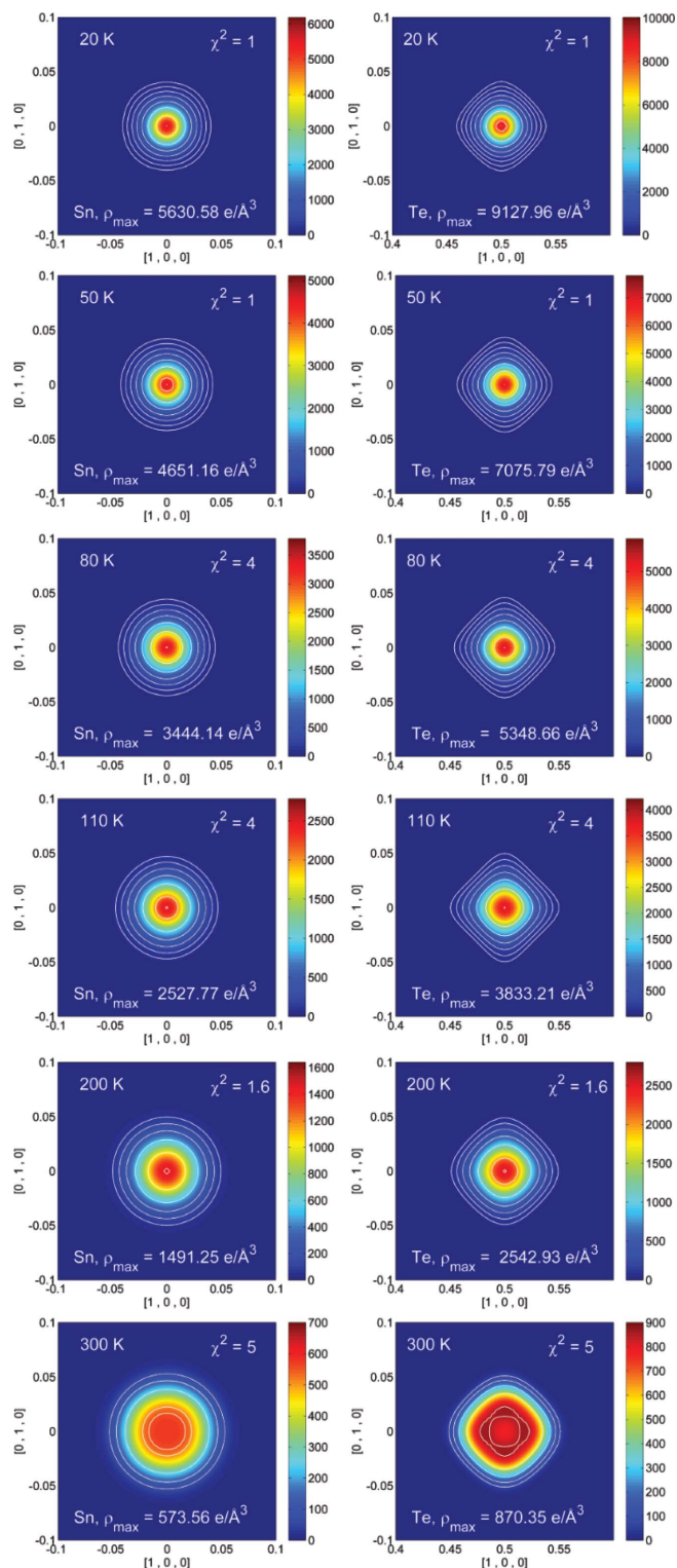
Figure 8 NXMEM electron-density maps for Sn (left) and Te (right) in the (001) plane from 20 to 300 K for sample B . Contour lines have been set at 64, 128, 256, 512, 1024, 2048, 4096 and 8192 e Å -3 . An additional contour line has been added as guide to locate the maximum corresponding to the nuclear position.
