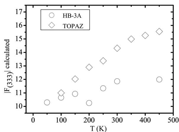
Figure 10 The temperature dependence of F_{333} on an absolute scale calculated from U_{\text{iso}}(\text{Sn}) and U_{\text{iso}}(\text{Te}) reported by Li, Ma et al. (2014)
