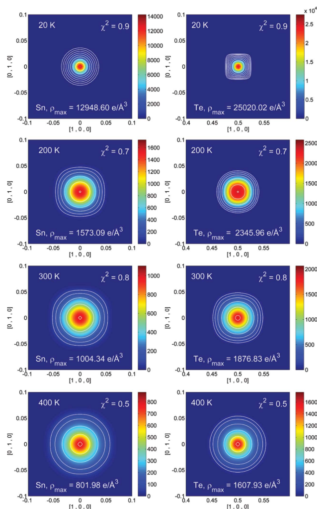
Figure 7 NXMEM electron-density maps for Sn (left) and Te (right) in the (001) plane from 20 to 400 K for sample A . Contour lines have been set at 64, 128, 256, 512, 1024, 2048, 4096 and 8192 e \text{ \AA}^{-3} . An additional contour line has been added as a guide to locate the maximum corresponding to the nuclear position.
