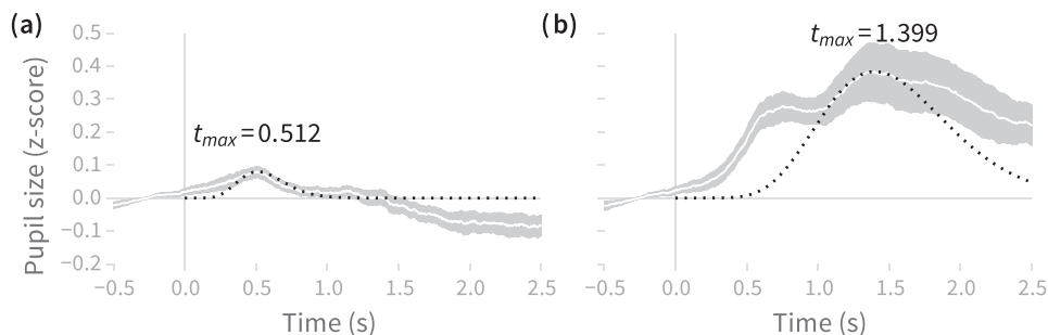
Fig. 1. Mean ( \pm 1 standard error) pupil size across subjects in response to (a) steady tones and (b) FM tones, with latency of maximum response ( t_{max} ) labeled. The late peak for FM tones is attributable to the behavioral response (button press) in those trials. Dark dotted lines show deconvolution kernels calculated from the different t_{max} values.
