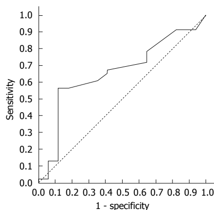
Figure 1 Receiver operating characteristic curve of omeprazole dose for recurrence.
